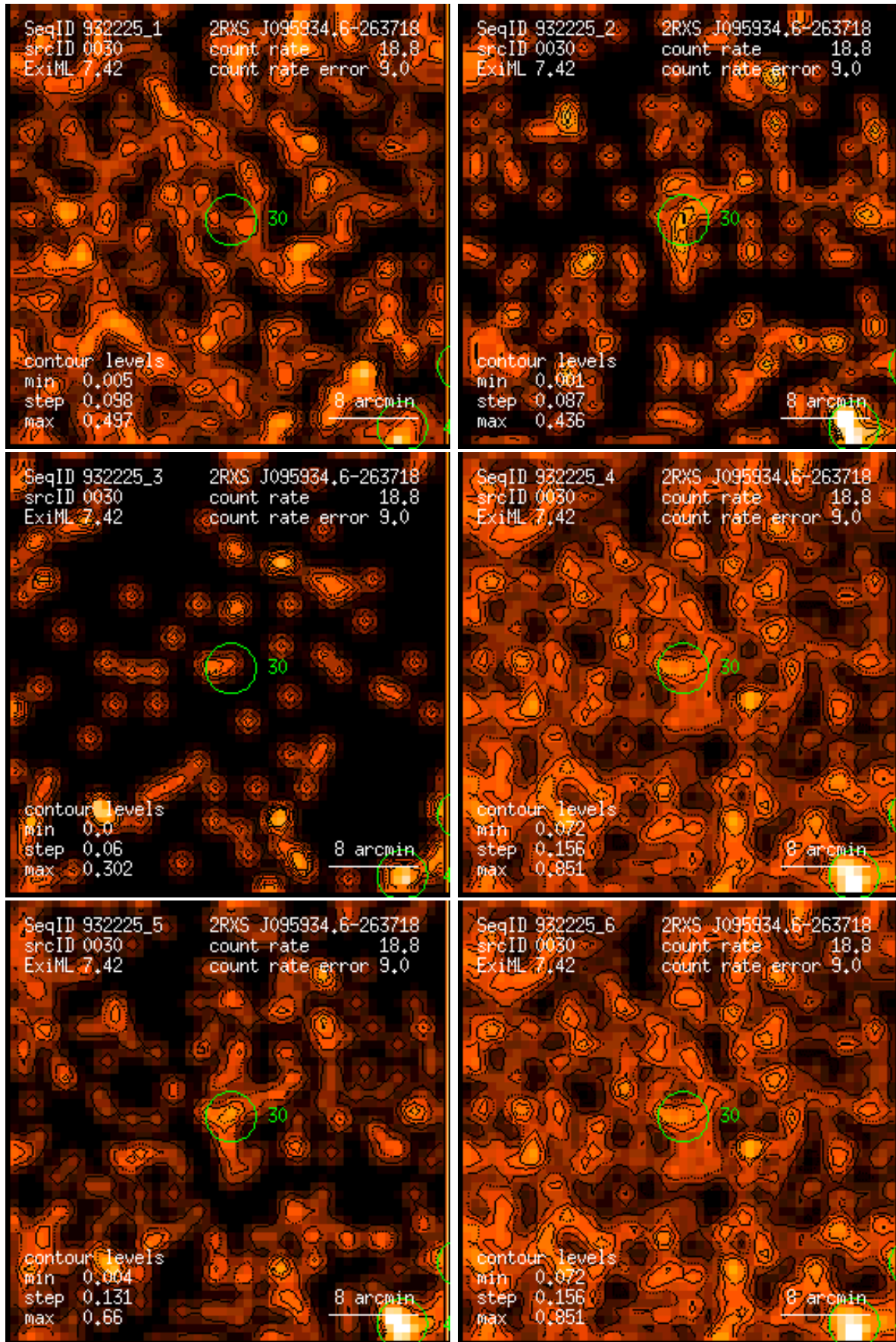
Figure 30: RASS 932225: detection 0030: band rate images, Gaussian filter: (1) PSPC channels 11 – 41, (2) 52 – 90, (3) 91 – 201, (4) 11 – 235, (5) 52 – 201, (6) 11 – 201. Broad band rates in counts/ks. Band rate contour levels in counts/ks/arcmin 2 .
