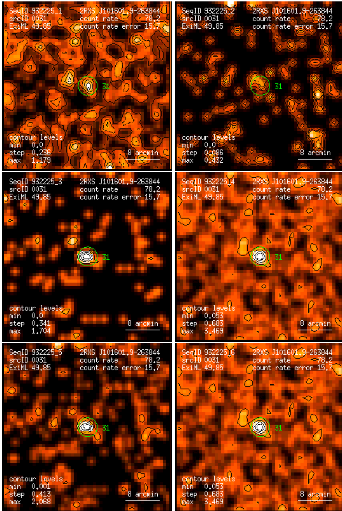
Figure 31: RASS 932225: detection 0031: band rate images, Gaussian filter: (1) PSPC channels 11 – 41, (2) 52 – 90, (3) 91 – 201, (4) 11 – 235, (5) 52 – 201, (6) 11 – 201. Broad band rates in counts/ks. Band rate contour levels in counts/ks/arcmin 2 .
