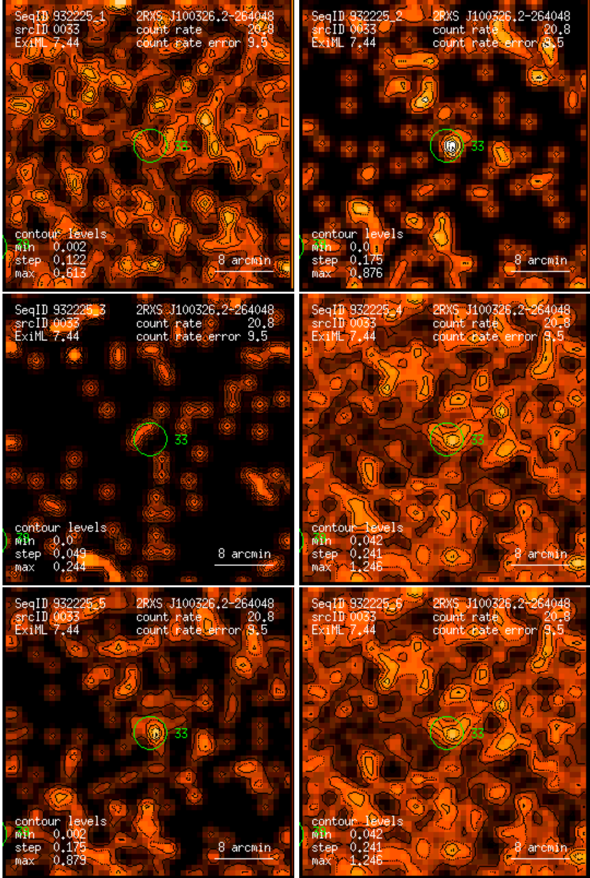
Figure 33: RASS 932225: detection 0033: band rate images, Gaussian filter: (1) PSPC channels 11 – 41, (2) 52 – 90, (3) 91 – 201, (4) 11 – 235, (5) 52 – 201, (6) 11 – 201. Broad band rates in counts/ks. Band rate contour levels in counts/ks/arcmin 2 .
