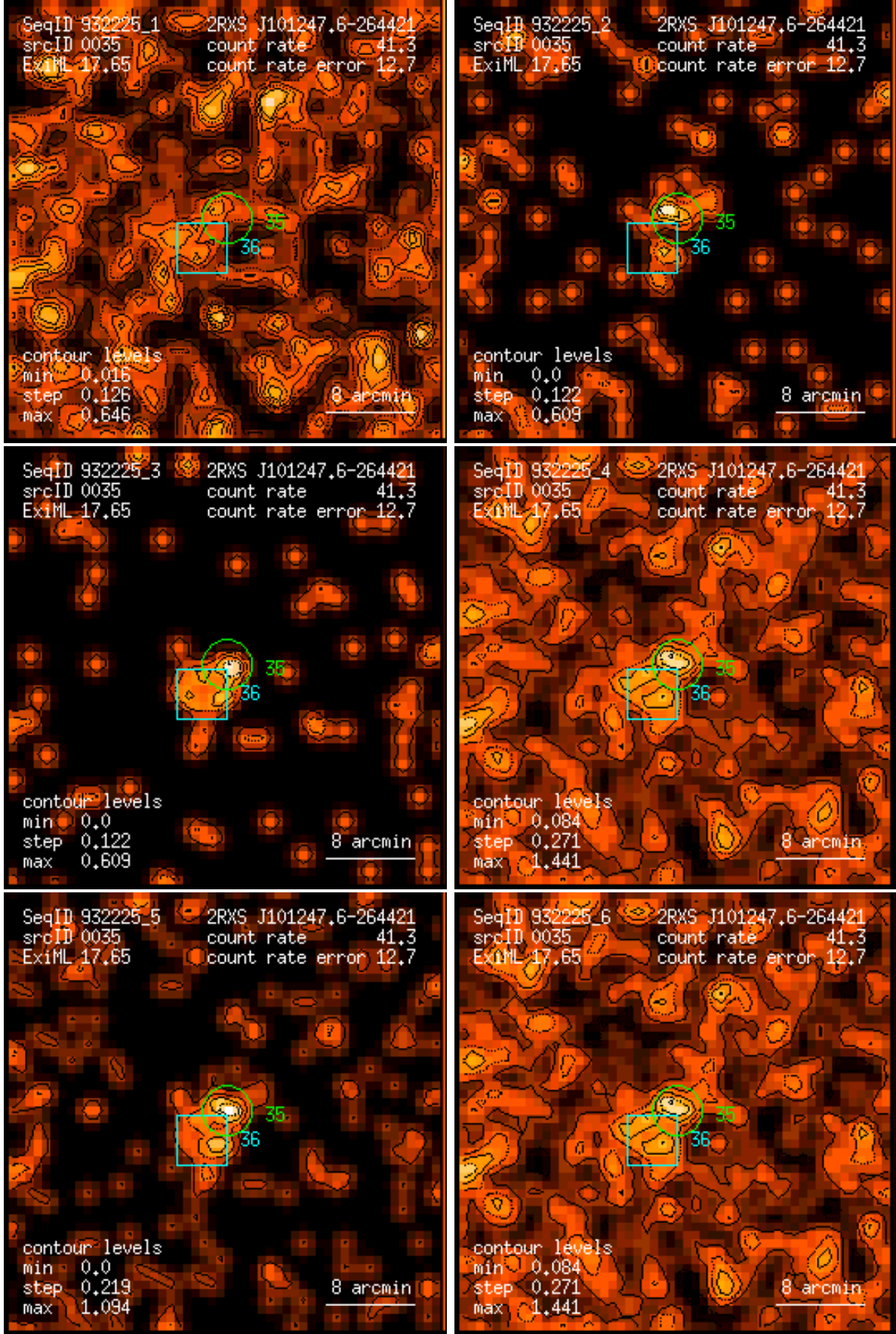
Figure 35: RASS 932225: detection 0035: band rate images, Gaussian filter: (1) PSPC channels 11 – 41, (2) 52 – 90, (3) 91 – 201, (4) 11 – 235, (5) 52 – 201, (6) 11 – 201. Broad band rates in counts/ks. Band rate contour levels in counts/ks/arcmin 2 .
