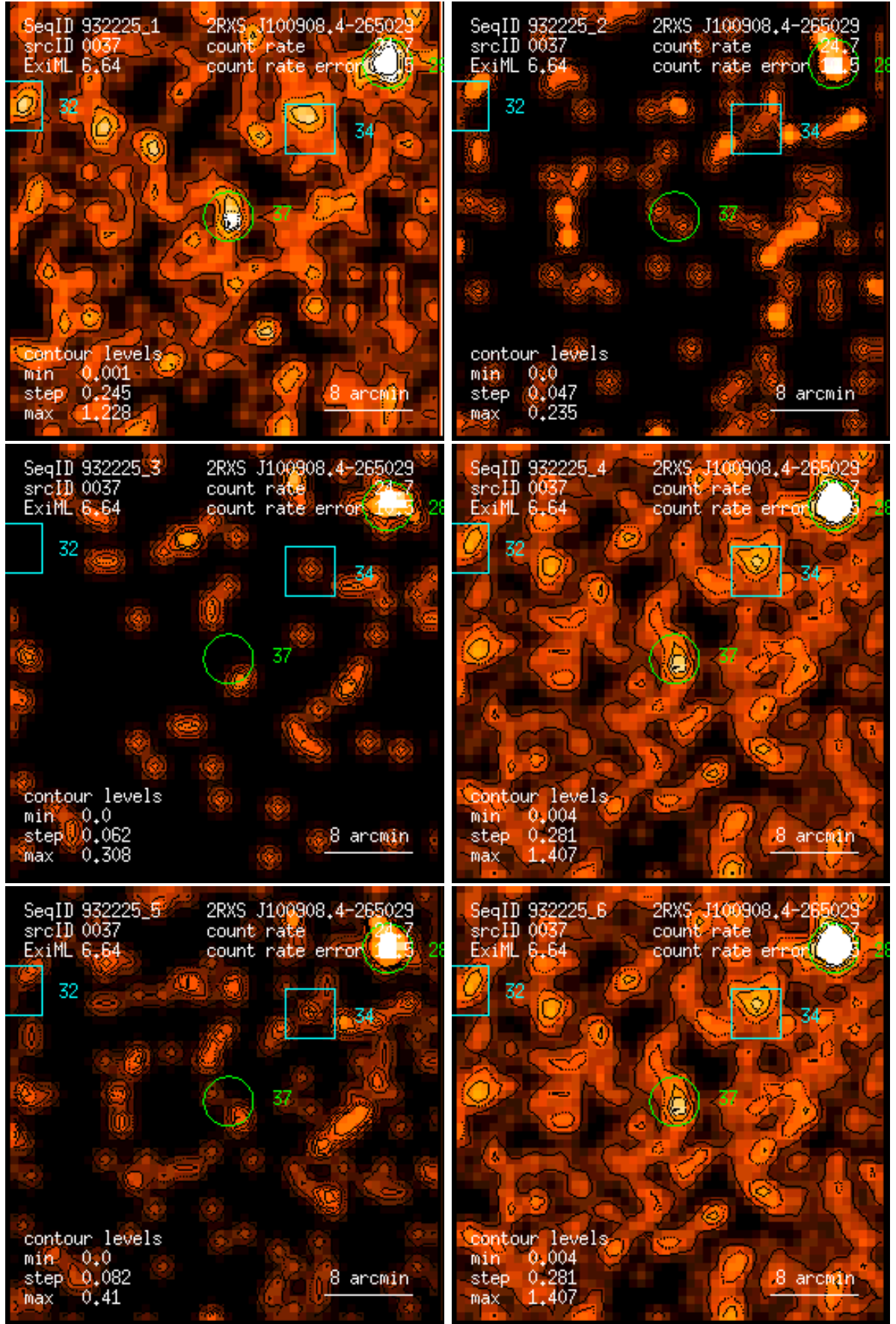
Figure 37: RASS 932225: detection 0037: band rate images, Gaussian filter: (1) PSPC channels 11 – 41, (2) 52 – 90, (3) 91 – 201, (4) 11 – 235, (5) 52 – 201, (6) 11 – 201. Broad band rates in counts/ks. Band rate contour levels in counts/ks/arcmin 2 .
