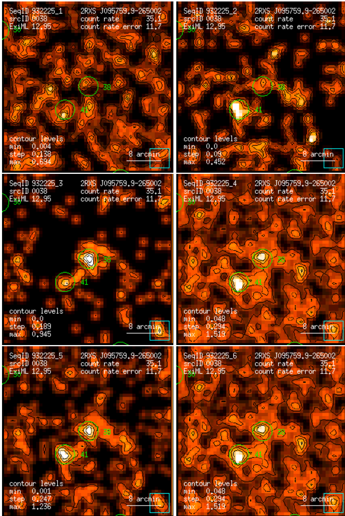
Figure 38: RASS 932225: detection 0038: band rate images, Gaussian filter: (1) PSPC channels 11 – 41, (2) 52 – 90, (3) 91 – 201, (4) 11 – 235, (5) 52 – 201, (6) 11 – 201. Broad band rates in counts/ks. Band rate contour levels in counts/ks/arcmin 2 .
