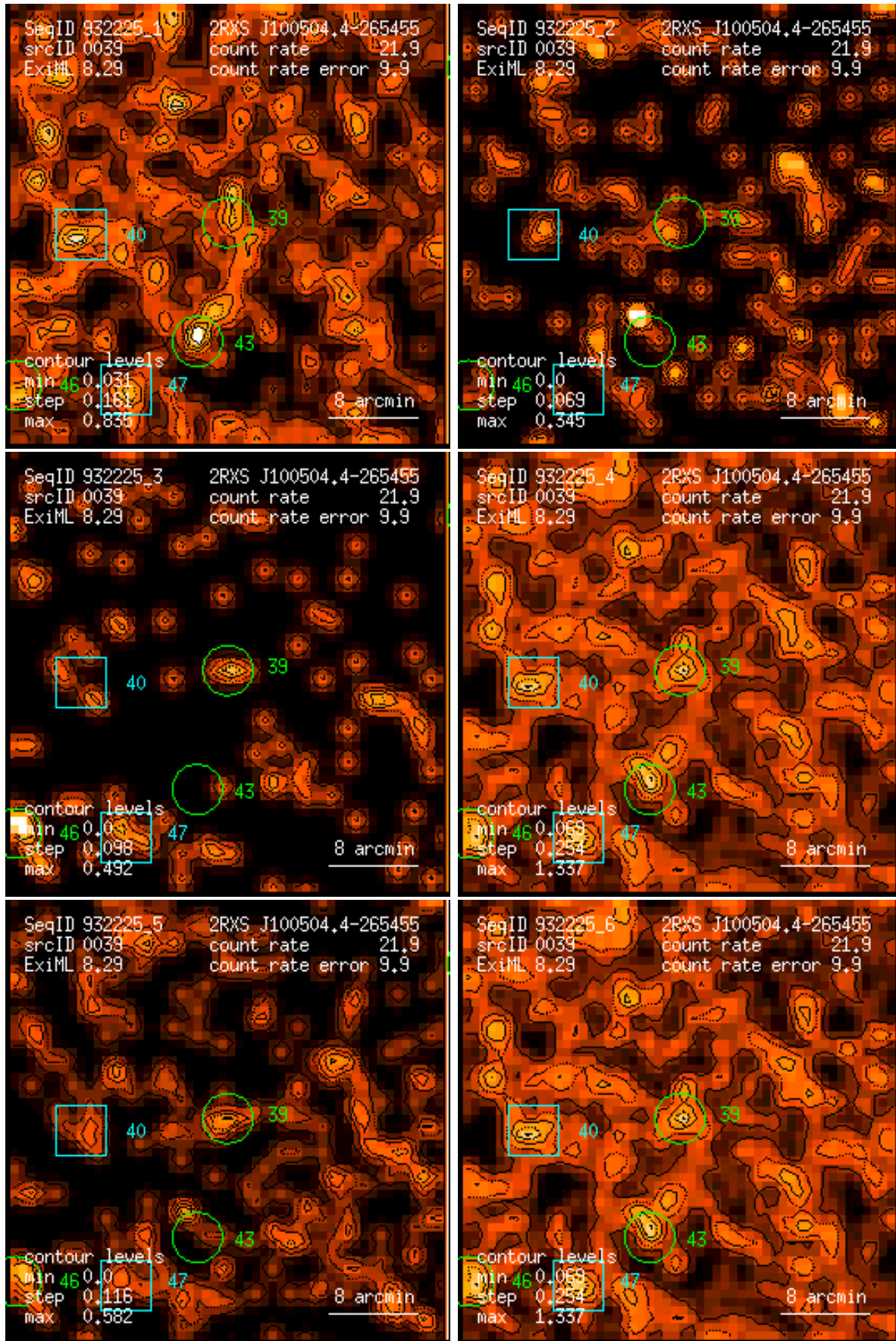
Figure 39: RASS 932225: detection 0039: band rate images, Gaussian filter: (1) PSPC channels 11 – 41, (2) 52 – 90, (3) 91 – 201, (4) 11 – 235, (5) 52 – 201, (6) 11 – 201. Broad band rates in counts/ks. Band rate contour levels in counts/ks/arcmin 2 .
