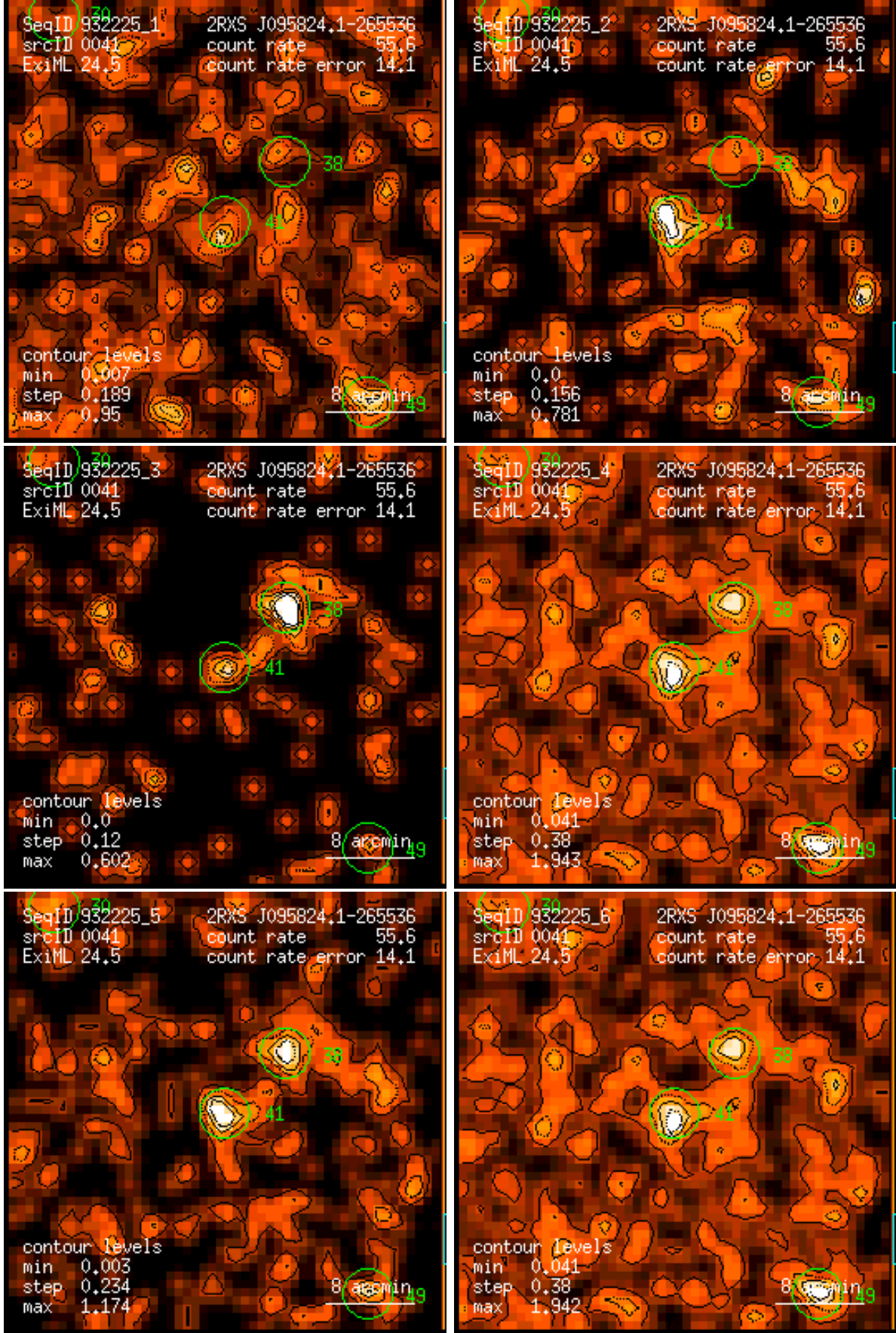
Figure 41: RASS 932225: detection 0041: band rate images, Gaussian filter: (1) PSPC channels 11 – 41, (2) 52 – 90, (3) 91 – 201, (4) 11 – 235, (5) 52 – 201, (6) 11 – 201. Broad band rates in counts/ks. Band rate contour levels in counts/ks/arcmin 2 .
