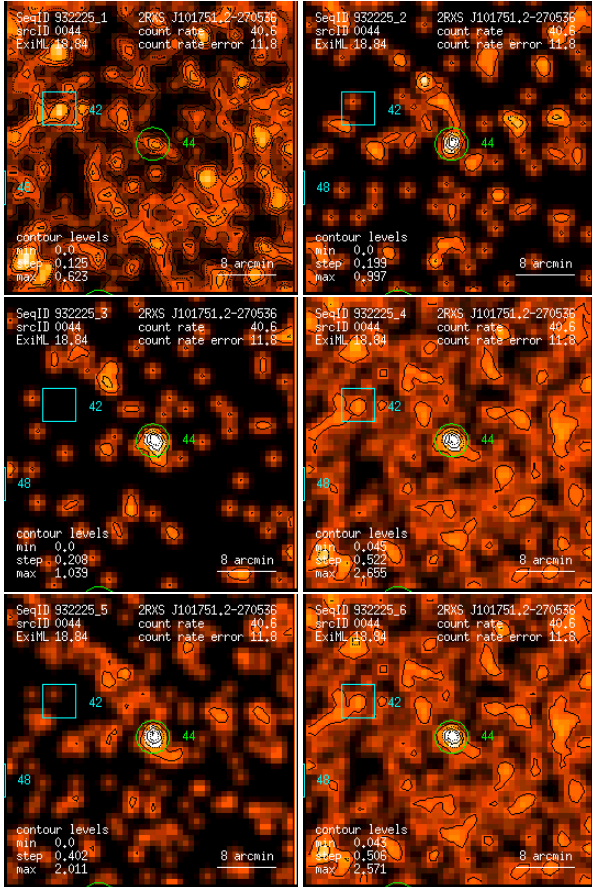
Figure 44: RASS 932225: detection 0044: band rate images, Gaussian filter: (1) PSPC channels 11 – 41, (2) 52 – 90, (3) 91 – 201, (4) 11 – 235, (5) 52 – 201, (6) 11 – 201. Broad band rates in counts/ks. Band rate contour levels in counts/ks/arcmin 2 .
