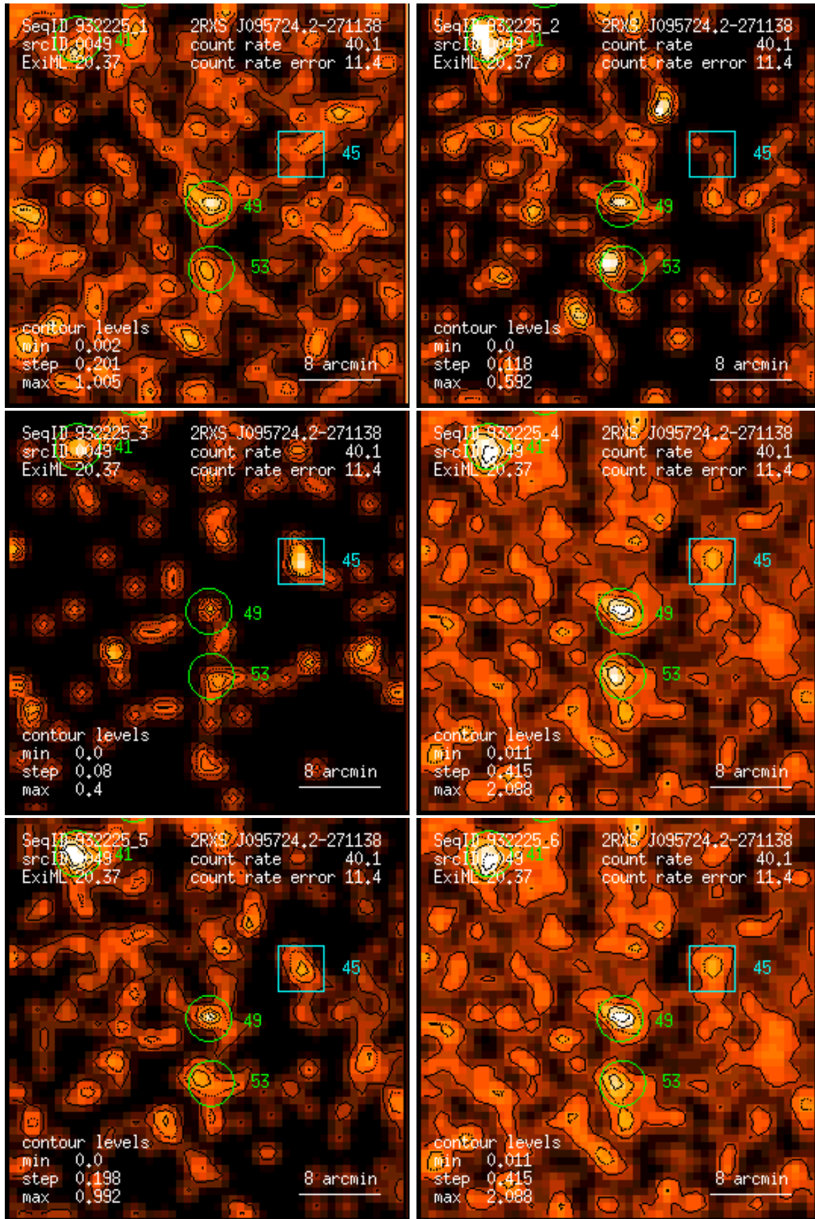
Figure 49: RASS 932225: detection 0049: band rate images, Gaussian filter: (1) PSPC channels 11 – 41, (2) 52 – 90, (3) 91 – 201, (4) 11 – 235, (5) 52 – 201, (6) 11 – 201. Broad band rates in counts/ks. Band rate contour levels in counts/ks/arcmin 2 .
