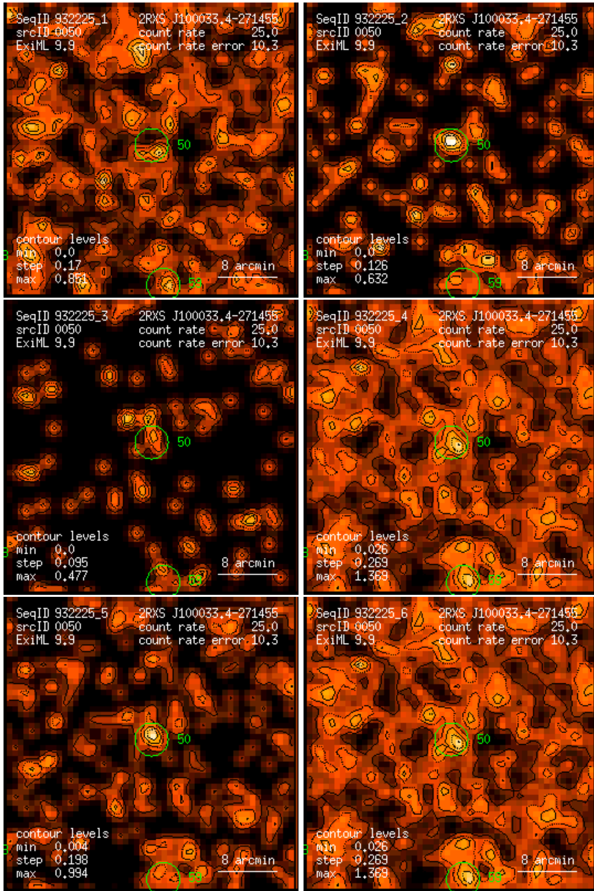
Figure 50: RASS 932225: detection 0050: band rate images, Gaussian filter: (1) PSPC channels 11 – 41, (2) 52 – 90, (3) 91 – 201, (4) 11 – 235, (5) 52 – 201, (6) 11 – 201. Broad band rates in counts/ks. Band rate contour levels in counts/ks/arcmin 2 .
