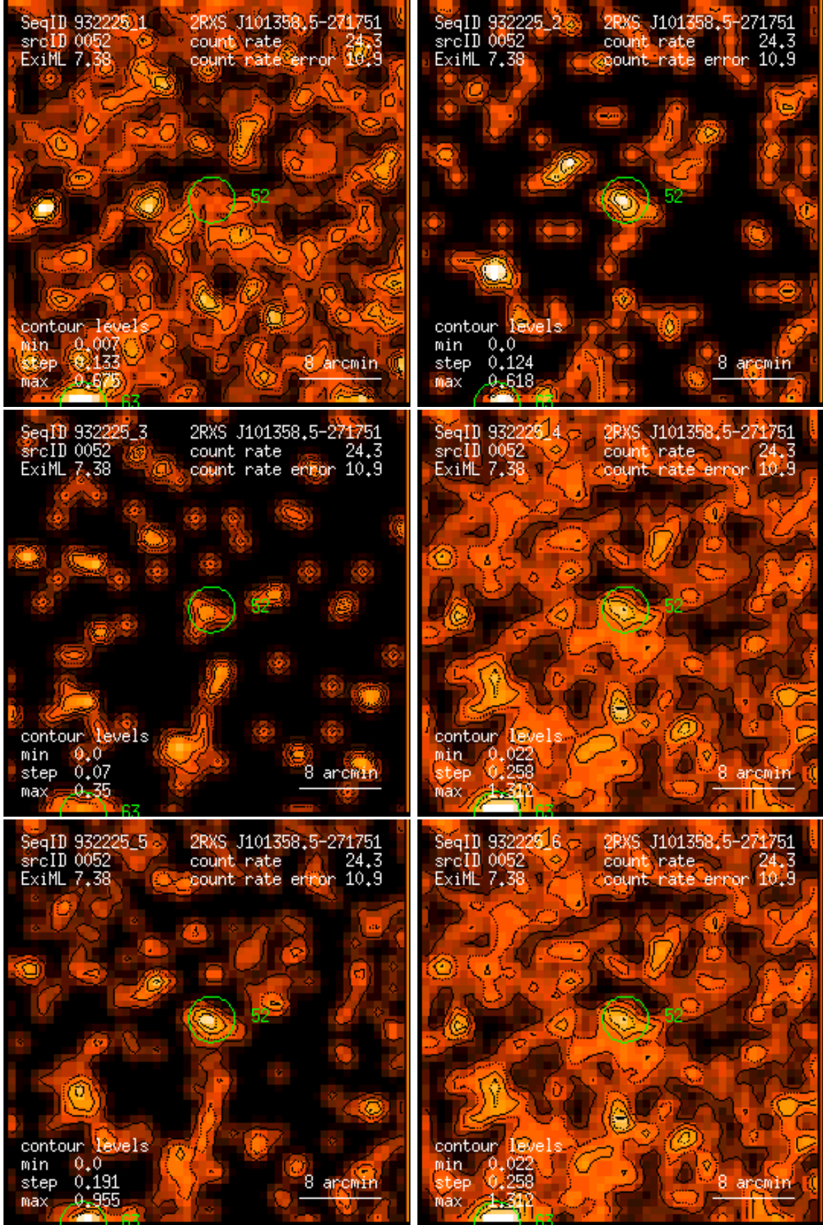
Figure 52: RASS 932225: detection 0052: band rate images, Gaussian filter: (1) PSPC channels 11 – 41, (2) 52 – 90, (3) 91 – 201, (4) 11 – 235, (5) 52 – 201, (6) 11 – 201. Broad band rates in counts/ks. Band rate contour levels in counts/ks/arcmin 2 .
