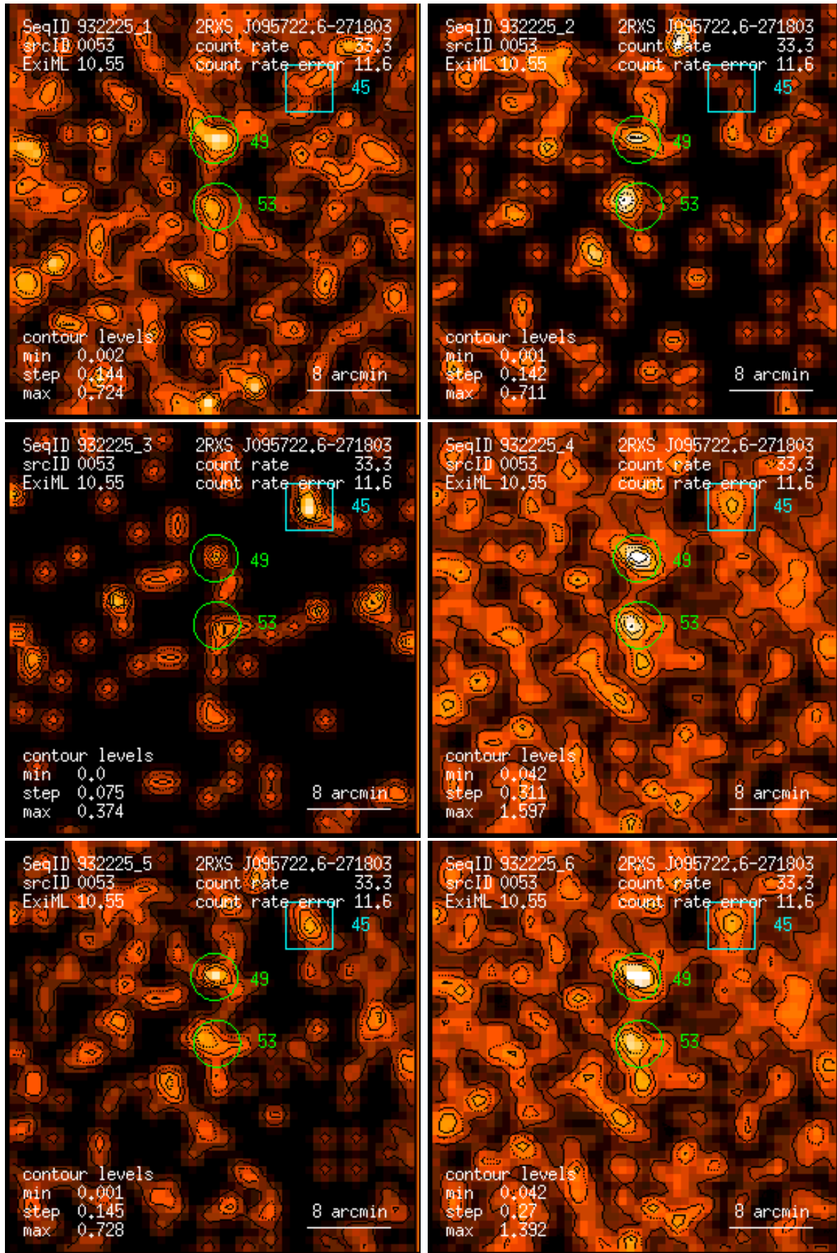
Figure 53: RASS 932225: detection 0053: band rate images, Gaussian filter: (1) PSPC channels 11 – 41, (2) 52 – 90, (3) 91 – 201, (4) 11 – 235, (5) 52 – 201, (6) 11 – 201. Broad band rates in counts/ks. Band rate contour levels in counts/ks/arcmin 2 .
