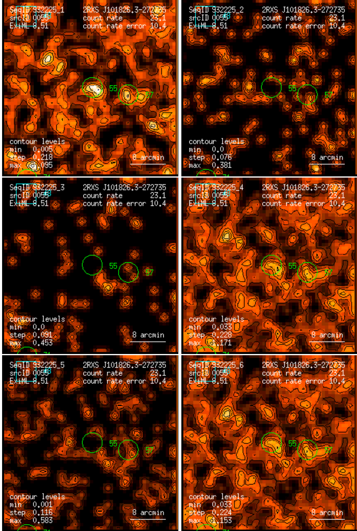
Figure 55: RASS 932225: detection 0055: band rate images, Gaussian filter: (1) PSPC channels 11 – 41, (2) 52 – 90, (3) 91 – 201, (4) 11 – 235, (5) 52 – 201, (6) 11 – 201. Broad band rates in counts/ks. Band rate contour levels in counts/ks/arcmin 2 .
