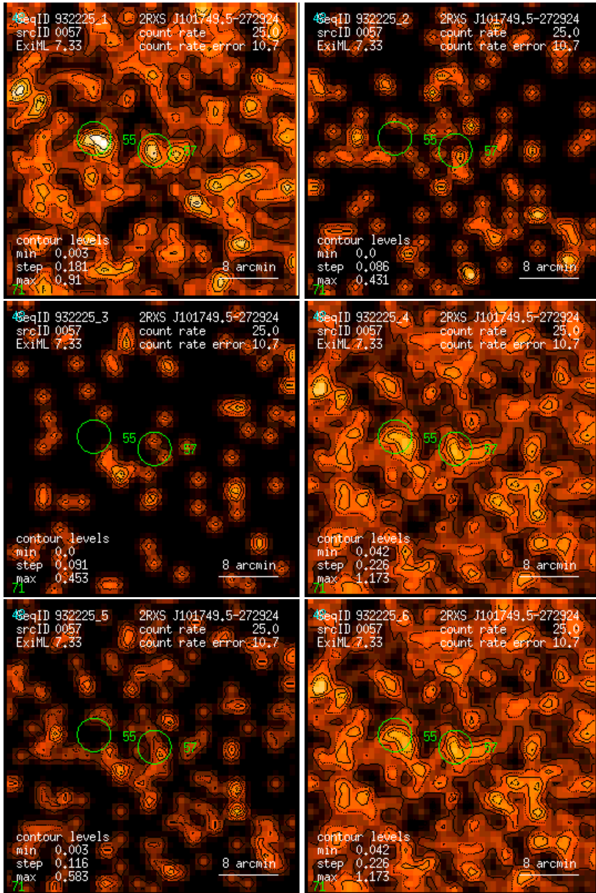
Figure 57: RASS 932225: detection 0057: band rate images, Gaussian filter: (1) PSPC channels 11 – 41, (2) 52 – 90, (3) 91 – 201, (4) 11 – 235, (5) 52 – 201, (6) 11 – 201. Broad band rates in counts/ks. Band rate contour levels in counts/ks/arcmin 2 .
