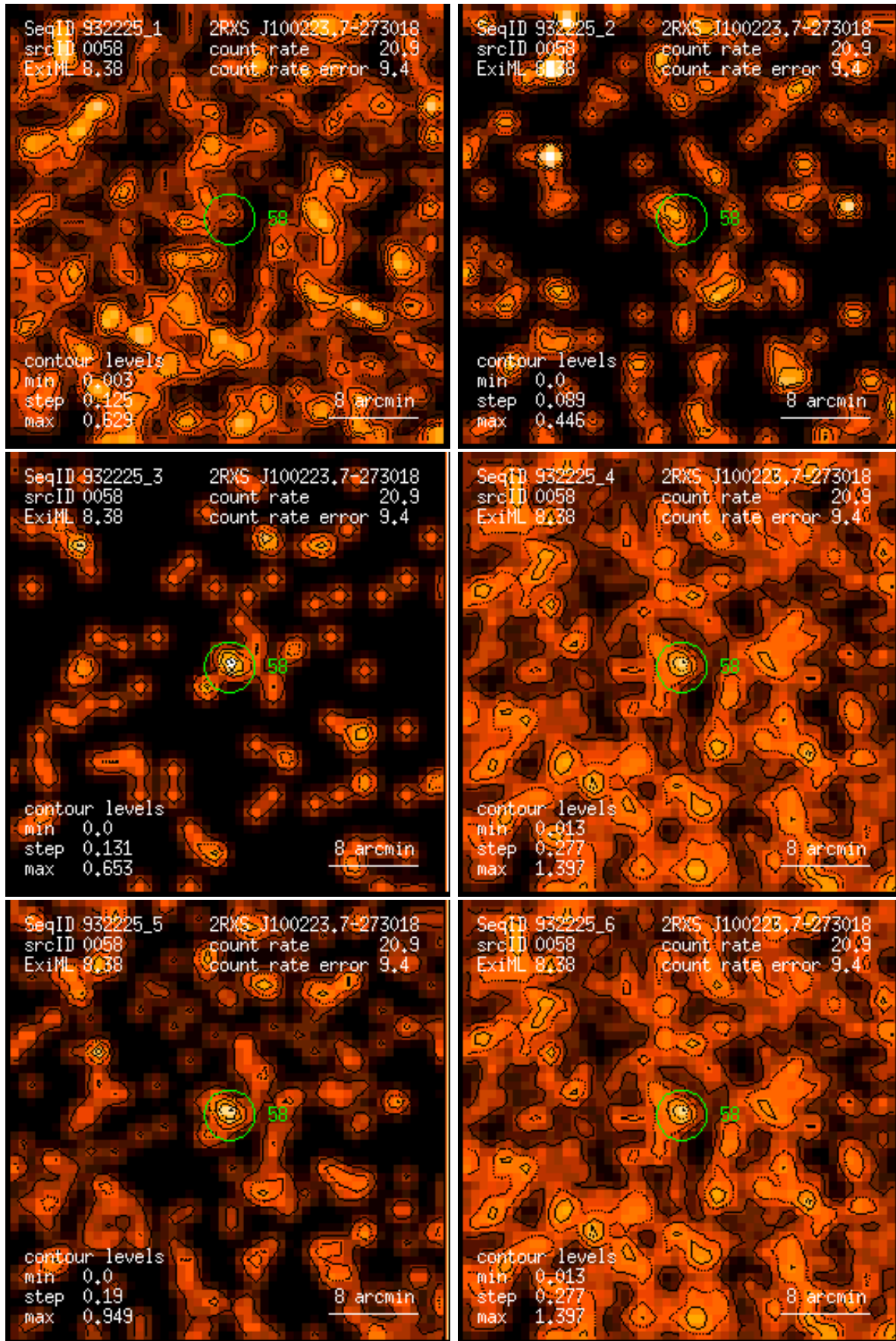
Figure 58: RASS 932225: detection 0058: band rate images, Gaussian filter: (1) PSPC channels 11 – 41, (2) 52 – 90, (3) 91 – 201, (4) 11 – 235, (5) 52 – 201, (6) 11 – 201. Broad band rates in counts/ks. Band rate contour levels in counts/ks/arcmin 2 .
