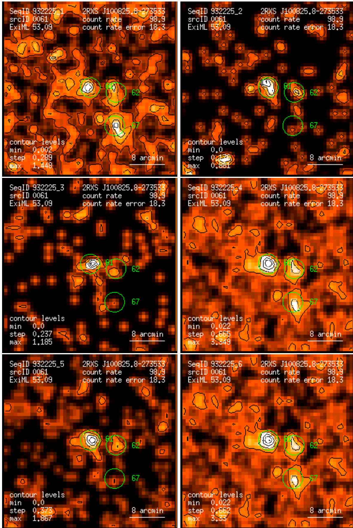
Figure 61: RASS 932225: detection 0061: band rate images, Gaussian filter: (1) PSPC channels 11 – 41, (2) 52 – 90, (3) 91 – 201, (4) 11 – 235, (5) 52 – 201, (6) 11 – 201. Broad band rates in counts/ks. Band rate contour levels in counts/ks/arcmin 2 .
