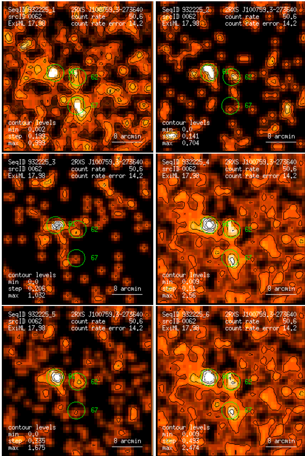
Figure 62: RASS 932225: detection 0062: band rate images, Gaussian filter: (1) PSPC channels 11 – 41, (2) 52 – 90, (3) 91 – 201, (4) 11 – 235, (5) 52 – 201, (6) 11 – 201. Broad band rates in counts/ks. Band rate contour levels in counts/ks/arcmin 2 .
