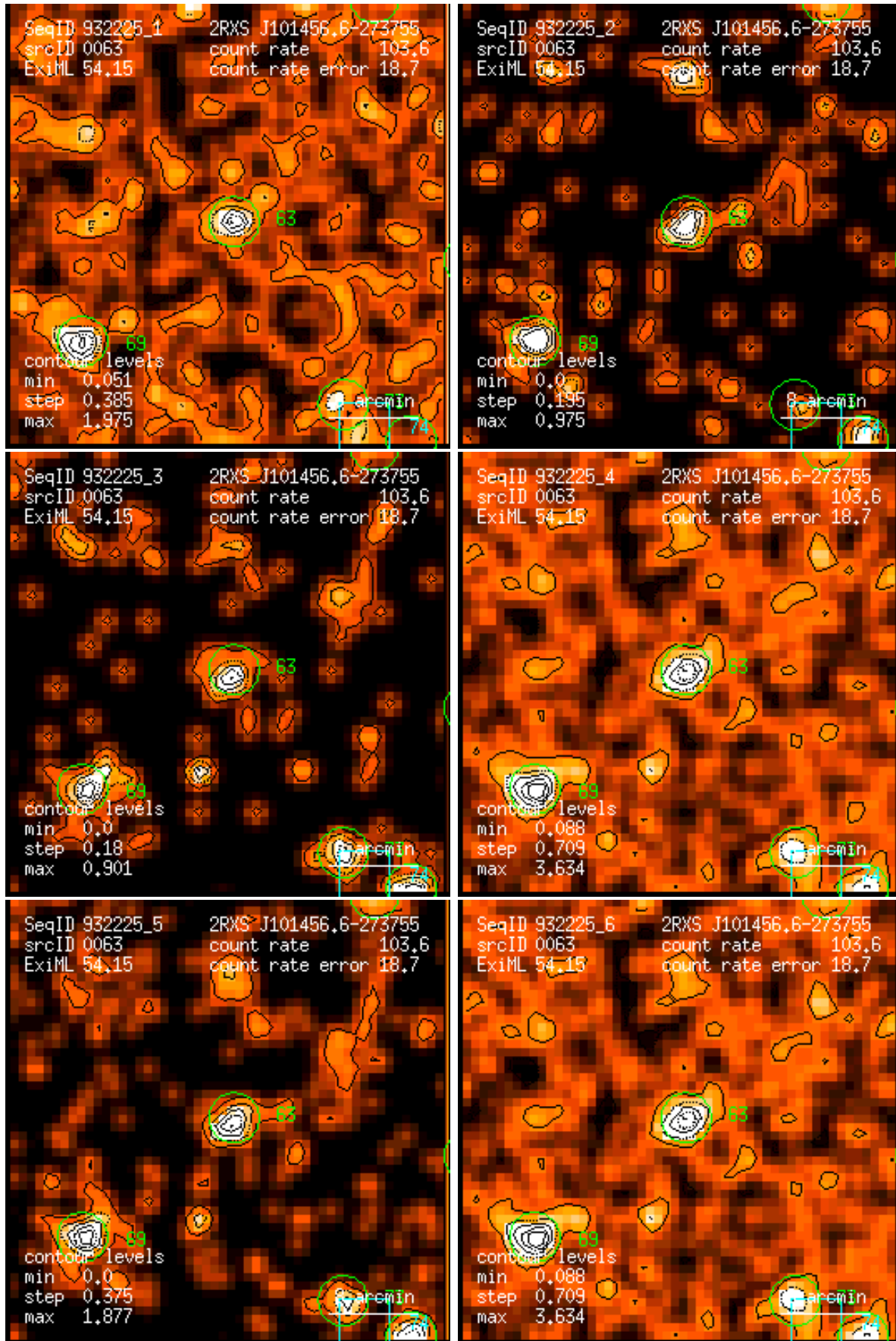
Figure 63: RASS 932225: detection 0063: band rate images, Gaussian filter: (1) PSPC channels 11 – 41, (2) 52 – 90, (3) 91 – 201, (4) 11 – 235, (5) 52 – 201, (6) 11 – 201. Broad band rates in counts/ks. Band rate contour levels in counts/ks/arcmin 2 .
