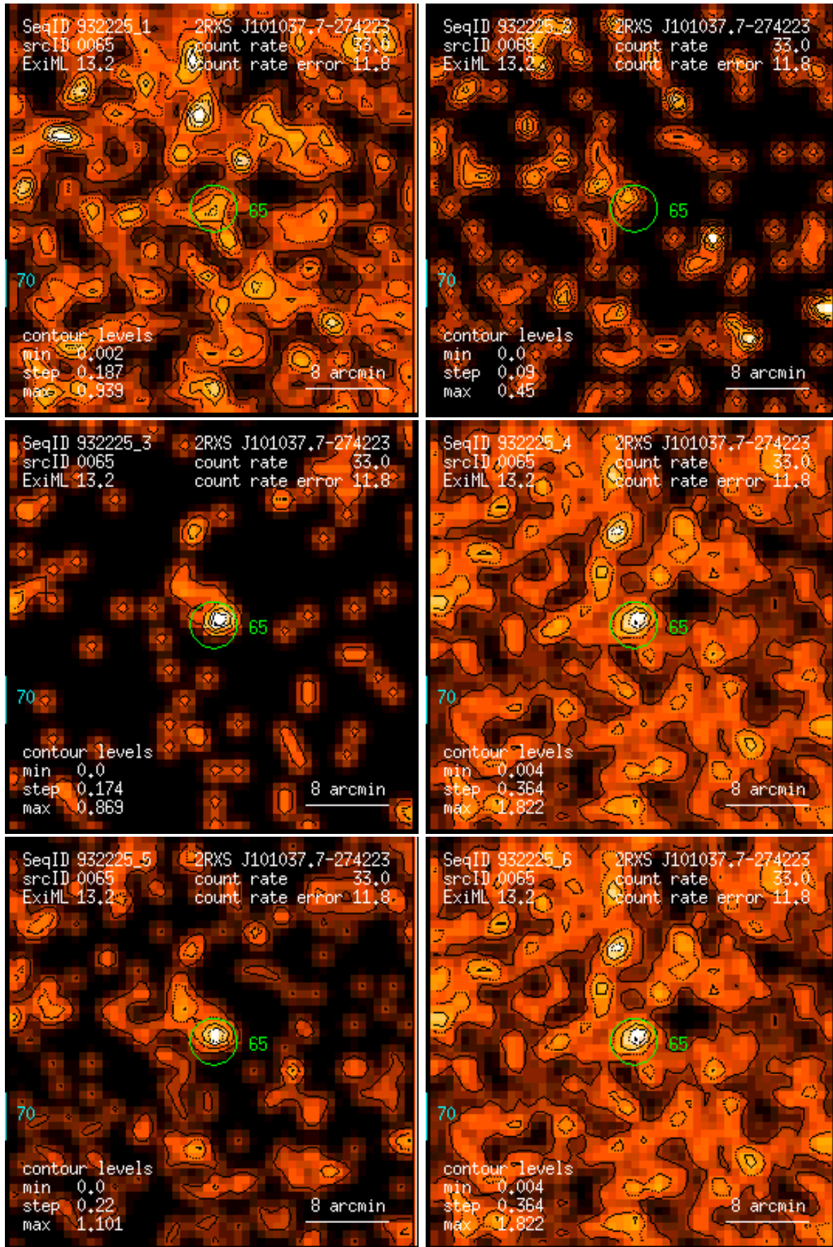
Figure 65: RASS 932225: detection 0065: band rate images, Gaussian filter: (1) PSPC channels 11 – 41, (2) 52 – 90, (3) 91 – 201, (4) 11 – 235, (5) 52 – 201, (6) 11 – 201. Broad band rates in counts/ks. Band rate contour levels in counts/ks/arcmin 2 .
