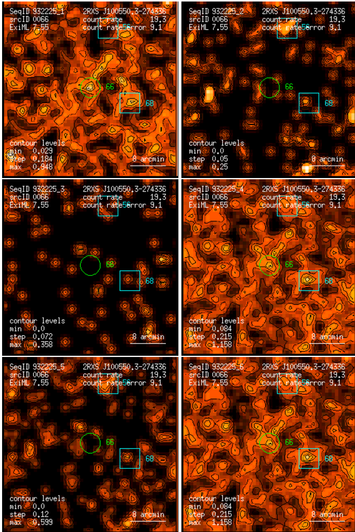
Figure 66: RASS 932225: detection 0066: band rate images, Gaussian filter: (1) PSPC channels 11 – 41, (2) 52 – 90, (3) 91 – 201, (4) 11 – 235, (5) 52 – 201, (6) 11 – 201. Broad band rates in counts/ks. Band rate contour levels in counts/ks/arcmin 2 .
