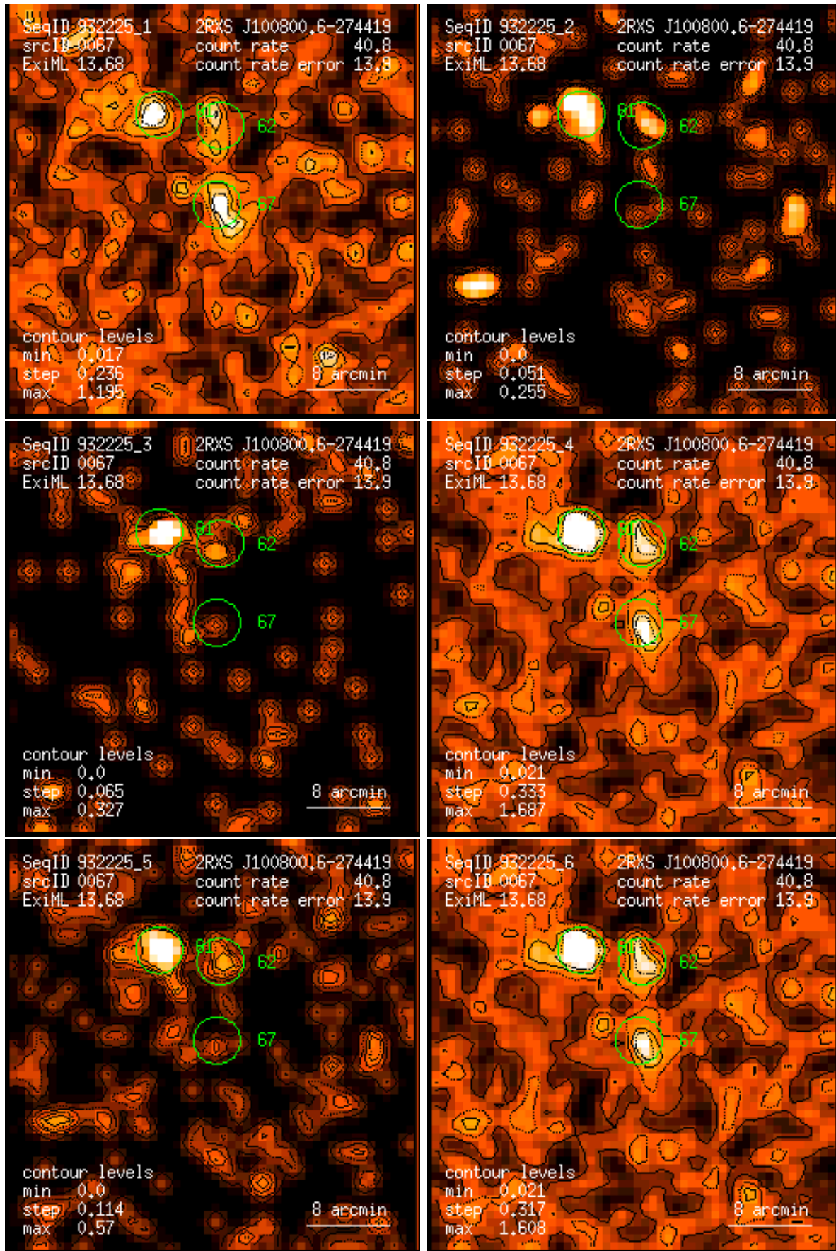
Figure 67: RASS 932225: detection 0067: band rate images, Gaussian filter: (1) PSPC channels 11 – 41, (2) 52 – 90, (3) 91 – 201, (4) 11 – 235, (5) 52 – 201, (6) 11 – 201. Broad band rates in counts/ks. Band rate contour levels in counts/ks/arcmin 2 .
