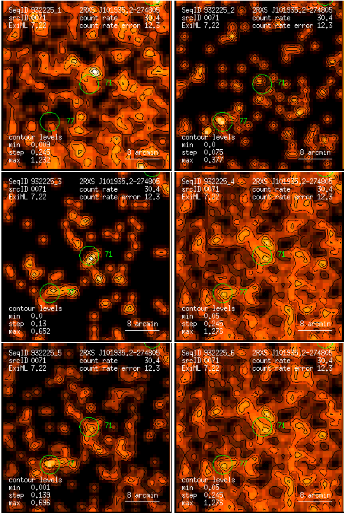
Figure 71: RASS 932225: detection 0071: band rate images, Gaussian filter: (1) PSPC channels 11 – 41, (2) 52 – 90, (3) 91 – 201, (4) 11 – 235, (5) 52 – 201, (6) 11 – 201. Broad band rates in counts/ks. Band rate contour levels in counts/ks/arcmin 2 .
