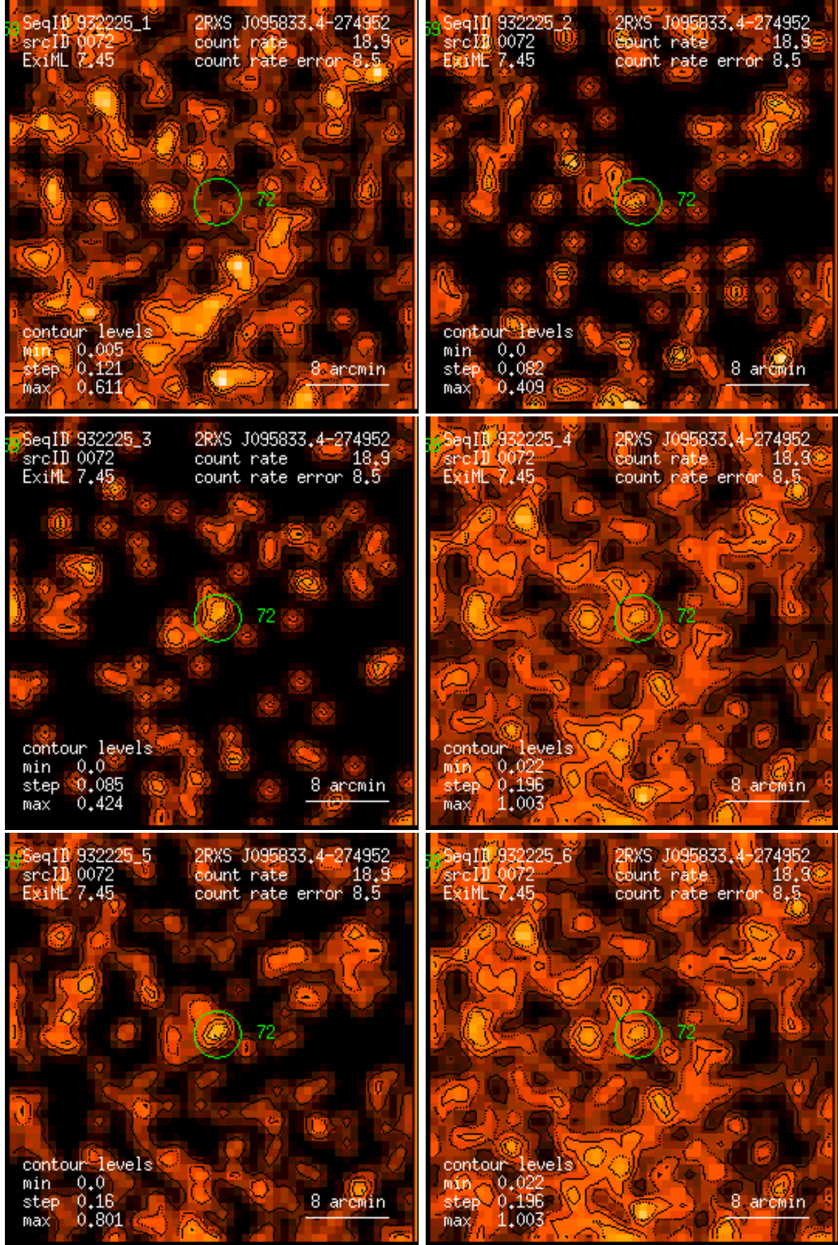
Figure 72: RASS 932225: detection 0072: band rate images, Gaussian filter: (1) PSPC channels 11 – 41, (2) 52 – 90, (3) 91 – 201, (4) 11 – 235, (5) 52 – 201, (6) 11 – 201. Broad band rates in counts/ks. Band rate contour levels in counts/ks/arcmin 2 .
