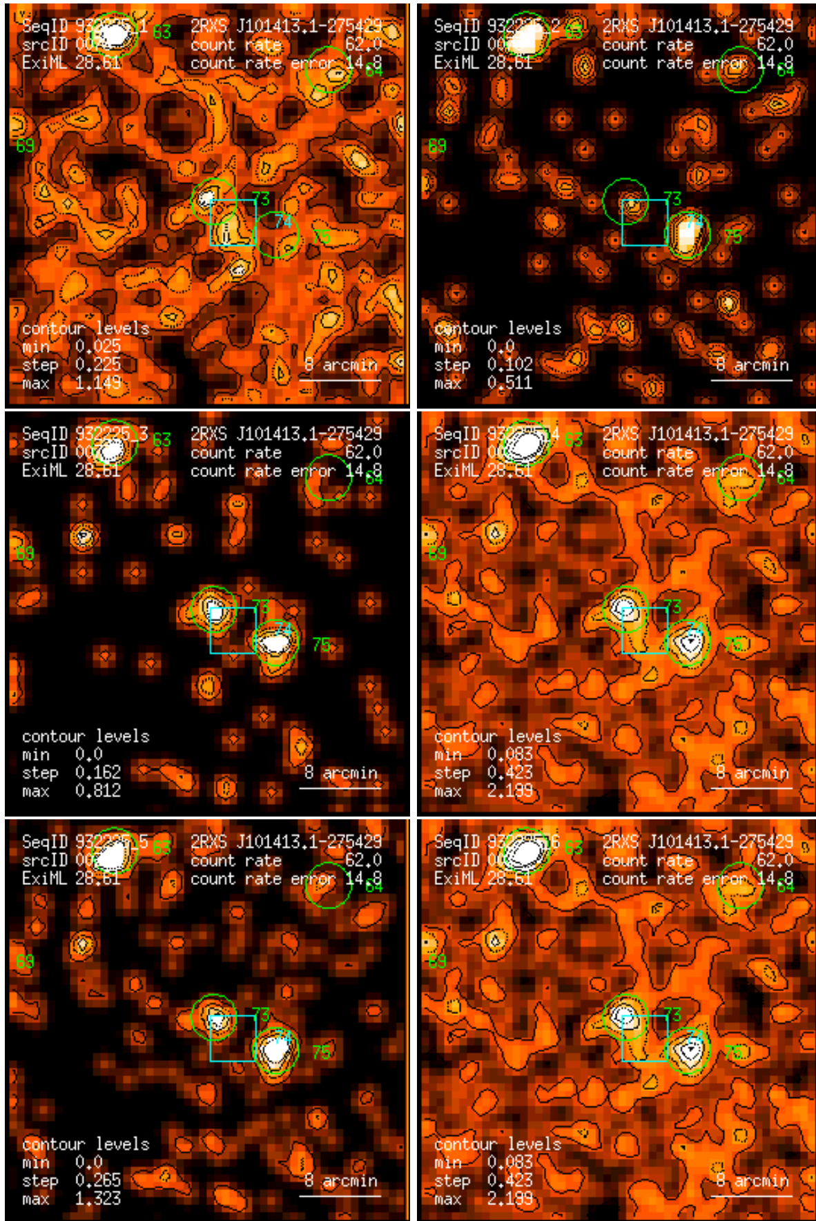
Figure 73: RASS 932225: detection 0073: band rate images, Gaussian filter: (1) PSPC channels 11 – 41, (2) 52 – 90, (3) 91 – 201, (4) 11 – 235, (5) 52 – 201, (6) 11 – 201. Broad band rates in counts/ks. Band rate contour levels in counts/ks/arcmin 2 .
