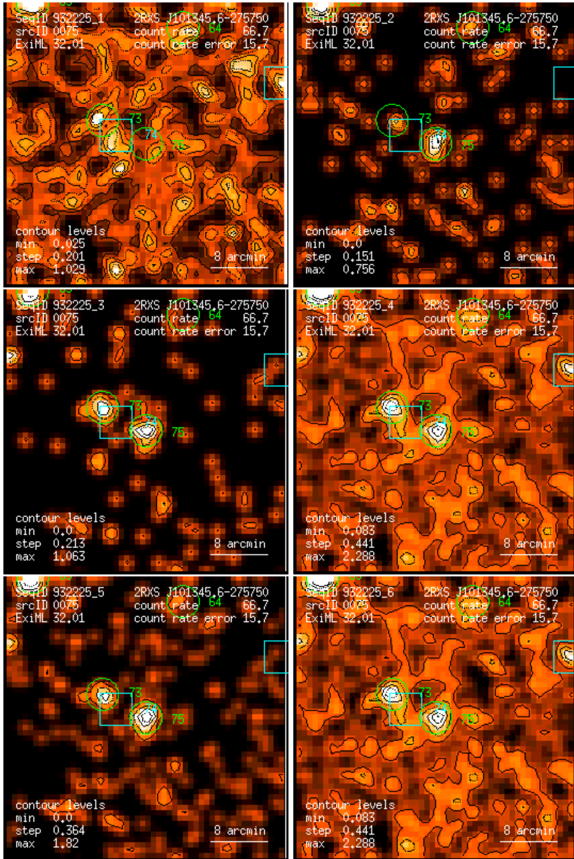
Figure 75: RASS 932225: detection 0075: band rate images, Gaussian filter: (1) PSPC channels 11 – 41, (2) 52 – 90, (3) 91 – 201, (4) 11 – 235, (5) 52 – 201, (6) 11 – 201. Broad band rates in counts/ks. Band rate contour levels in counts/ks/arcmin 2 .
