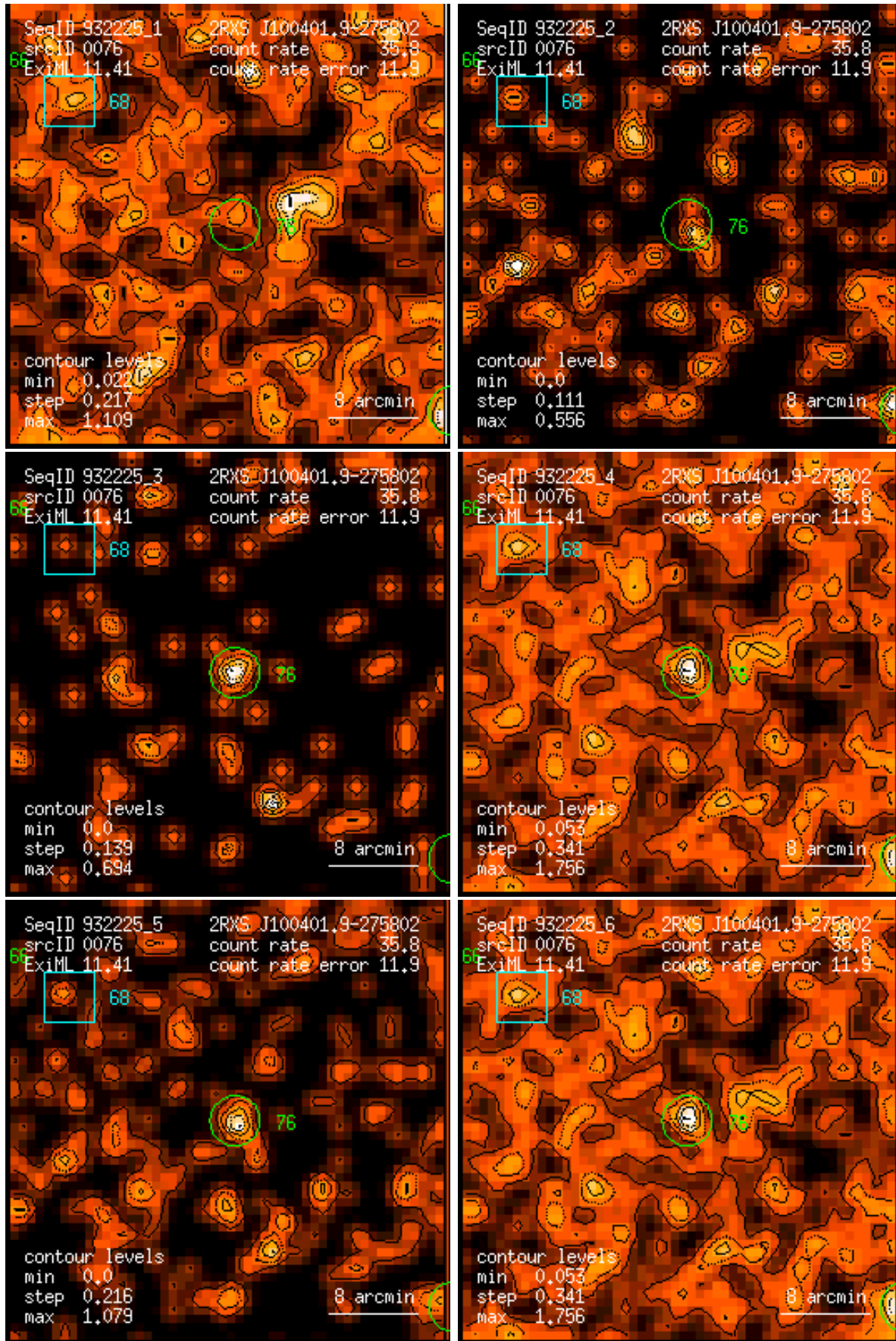
Figure 76: RASS 932225: detection 0076: band rate images, Gaussian filter: (1) PSPC channels 11 – 41, (2) 52 – 90, (3) 91 – 201, (4) 11 – 235, (5) 52 – 201, (6) 11 – 201. Broad band rates in counts/ks. Band rate contour levels in counts/ks/arcmin 2 .
