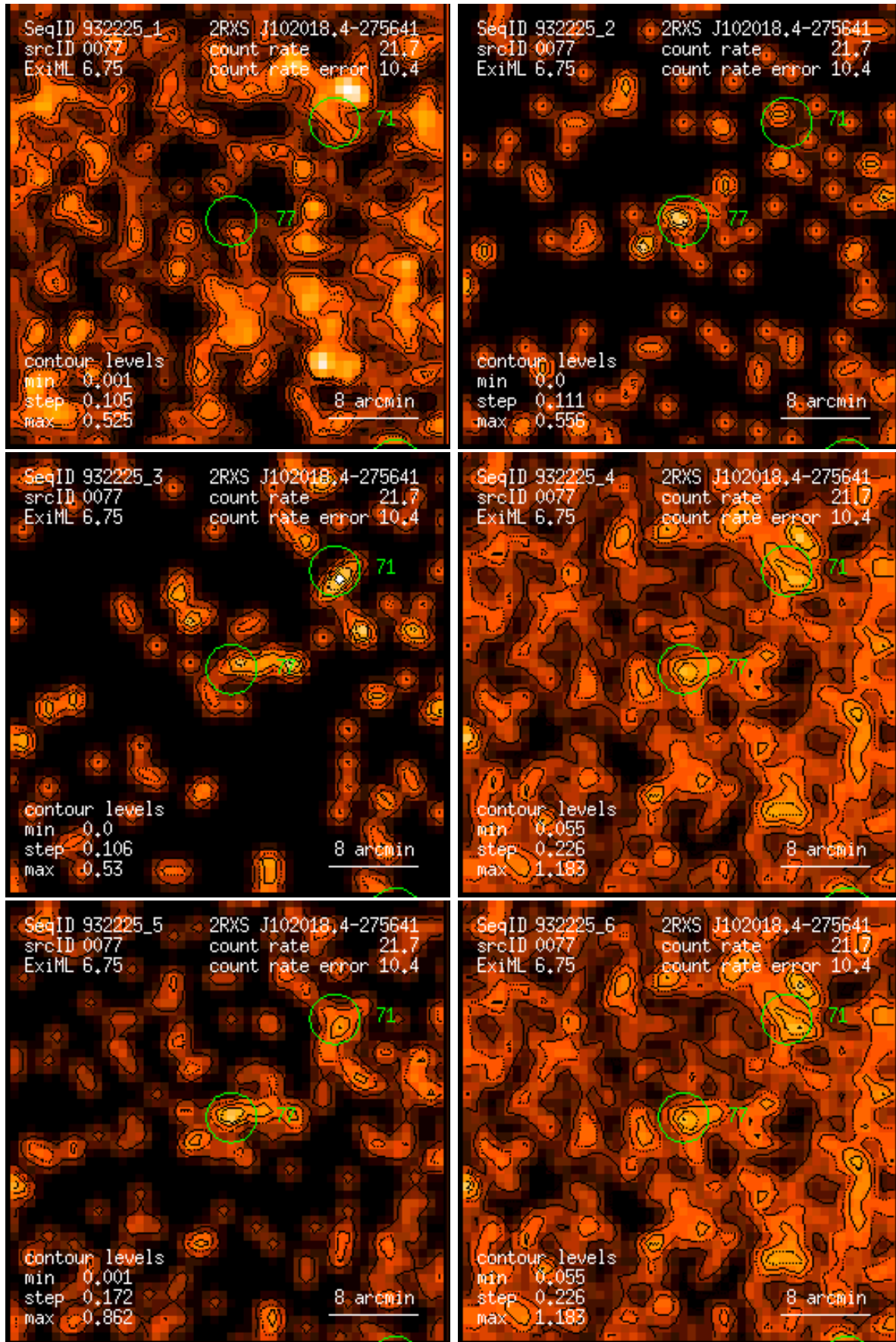
Figure 77: RASS 932225: detection 0077: band rate images, Gaussian filter: (1) PSPC channels 11 – 41, (2) 52 – 90, (3) 91 – 201, (4) 11 – 235, (5) 52 – 201, (6) 11 – 201. Broad band rates in counts/ks. Band rate contour levels in counts/ks/arcmin 2 .
