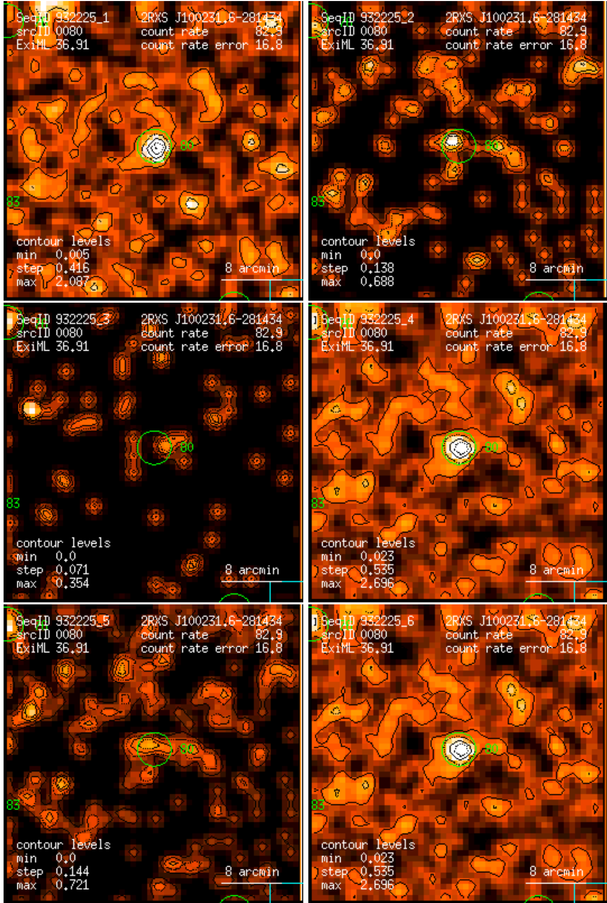
Figure 80: RASS 932225: detection 0080: band rate images, Gaussian filter: (1) PSPC channels 11 – 41, (2) 52 – 90, (3) 91 – 201, (4) 11 – 235, (5) 52 – 201, (6) 11 – 201. Broad band rates in counts/ks. Band rate contour levels in counts/ks/arcmin 2 .
