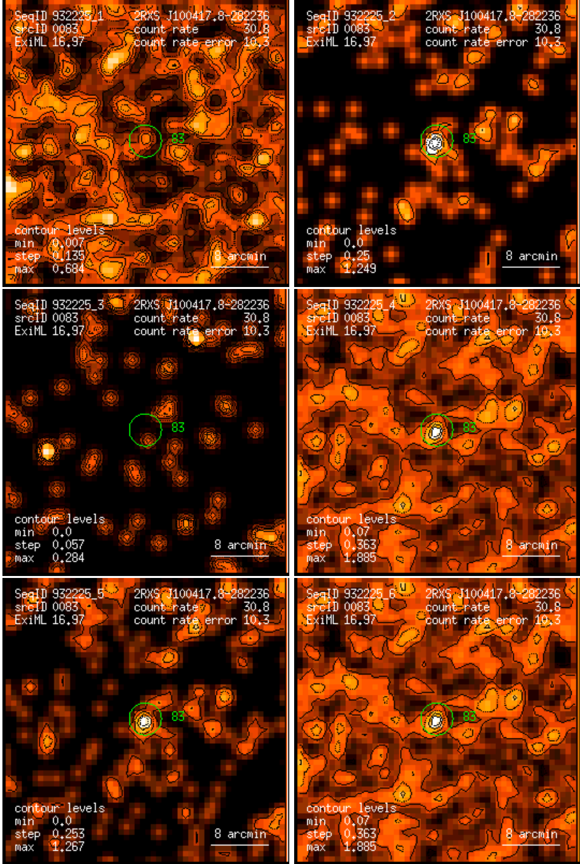
Figure 83: RASS 932225: detection 0083: band rate images, Gaussian filter: (1) PSPC channels 11 – 41, (2) 52 – 90, (3) 91 – 201, (4) 11 – 235, (5) 52 – 201, (6) 11 – 201. Broad band rates in counts/ks. Band rate contour levels in counts/ks/arcmin 2 .
