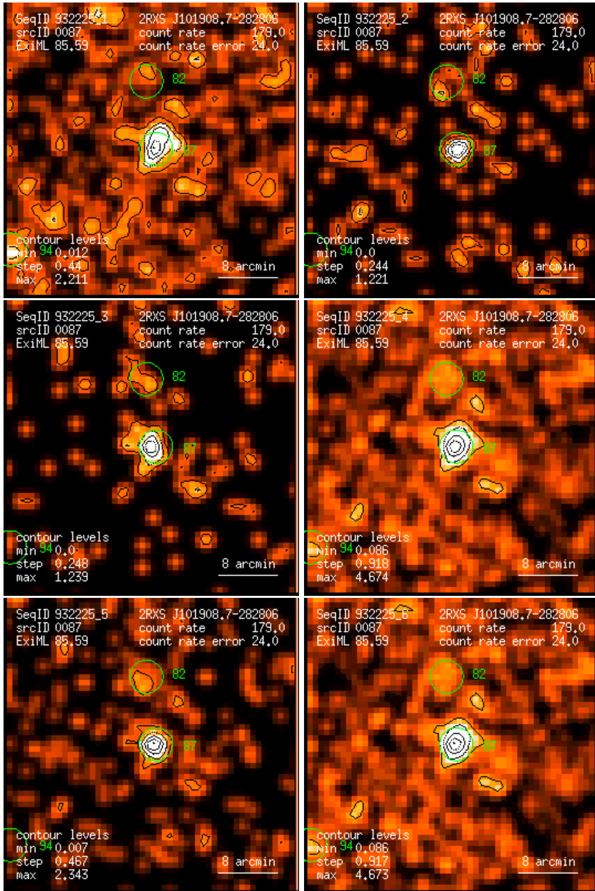
Figure 87: RASS 932225: detection 0087: band rate images, Gaussian filter: (1) PSPC channels 11 – 41, (2) 52 – 90, (3) 91 – 201, (4) 11 – 235, (5) 52 – 201, (6) 11 – 201. Broad band rates in counts/ks. Band rate contour levels in counts/ks/arcmin 2 .
