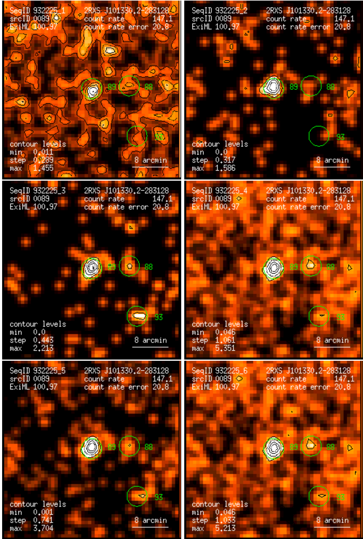
Figure 89: RASS 932225: detection 0089: band rate images, Gaussian filter: (1) PSPC channels 11 – 41, (2) 52 – 90, (3) 91 – 201, (4) 11 – 235, (5) 52 – 201, (6) 11 – 201. Broad band rates in counts/ks. Band rate contour levels in counts/ks/arcmin 2 .
