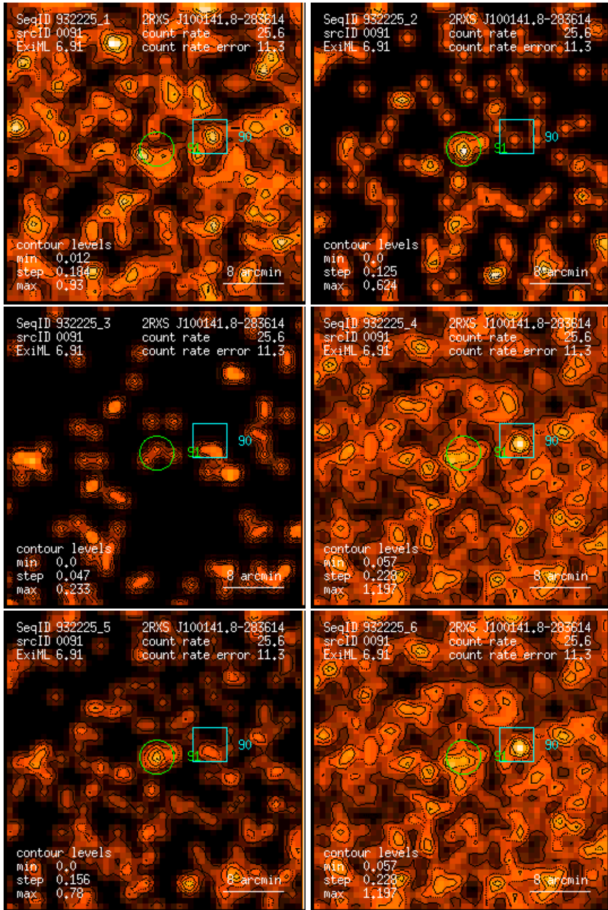
Figure 91: RASS 932225: detection 0091: band rate images, Gaussian filter: (1) PSPC channels 11 – 41, (2) 52 – 90, (3) 91 – 201, (4) 11 – 235, (5) 52 – 201, (6) 11 – 201. Broad band rates in counts/ks. Band rate contour levels in counts/ks/arcmin 2 .
