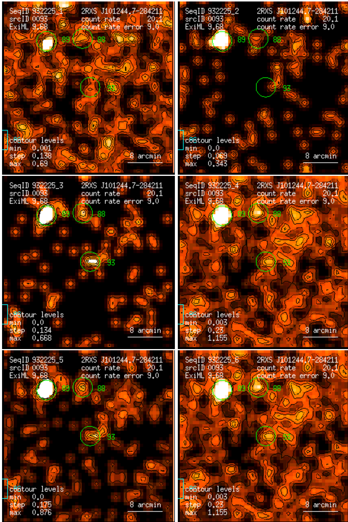
Figure 93: RASS 932225: detection 0093: band rate images, Gaussian filter: (1) PSPC channels 11 – 41, (2) 52 – 90, (3) 91 – 201, (4) 11 – 235, (5) 52 – 201, (6) 11 – 201. Broad band rates in counts/ks. Band rate contour levels in counts/ks/arcmin 2 .
