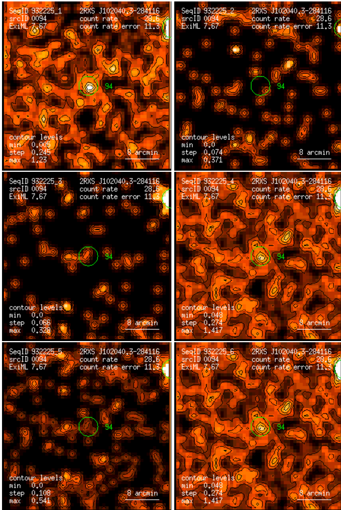
Figure 94: RASS 932225: detection 0094: band rate images, Gaussian filter: (1) PSPC channels 11 – 41, (2) 52 – 90, (3) 91 – 201, (4) 11 – 235, (5) 52 – 201, (6) 11 – 201. Broad band rates in counts/ks. Band rate contour levels in counts/ks/arcmin 2 .
