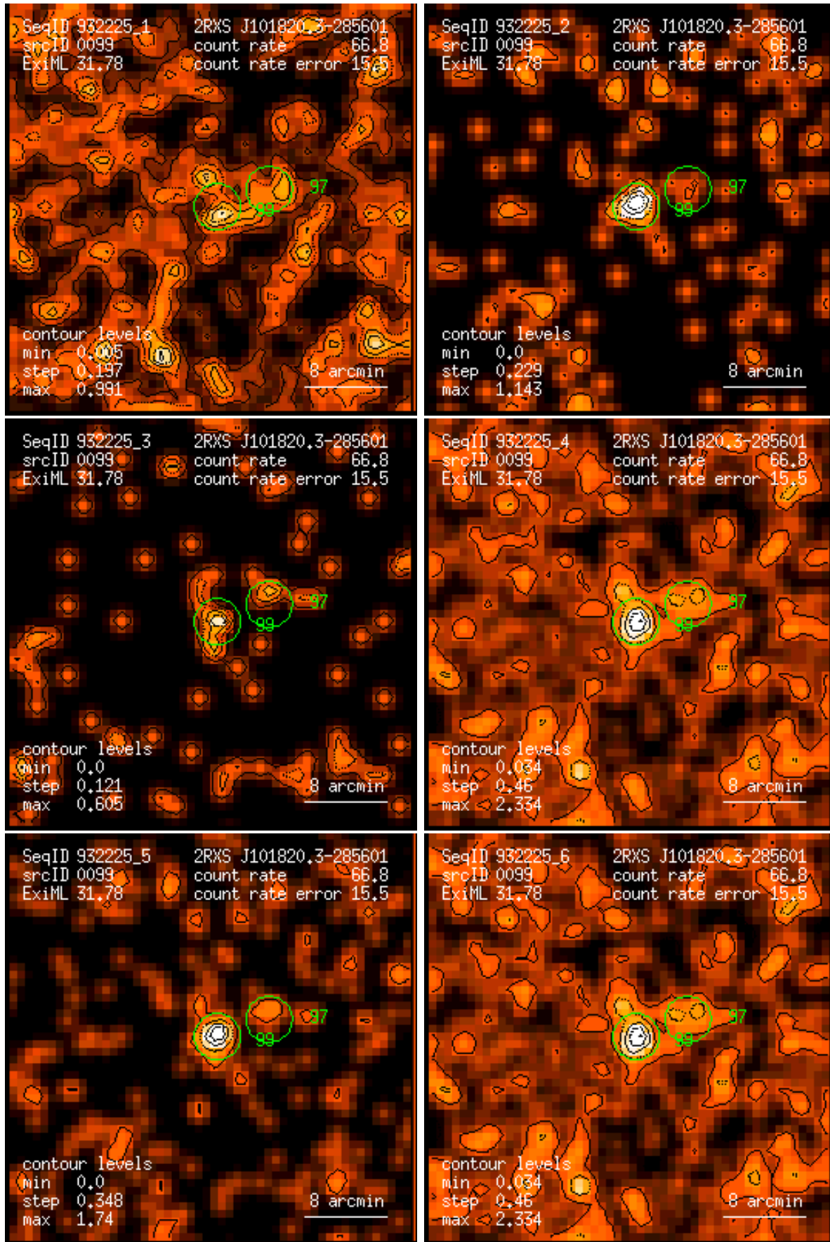
Figure 99: RASS 932225: detection 0099: band rate images, Gaussian filter: (1) PSPC channels 11 – 41, (2) 52 – 90, (3) 91 – 201, (4) 11 – 235, (5) 52 – 201, (6) 11 – 201. Broad band rates in counts/ks. Band rate contour levels in counts/ks/arcmin 2 .
