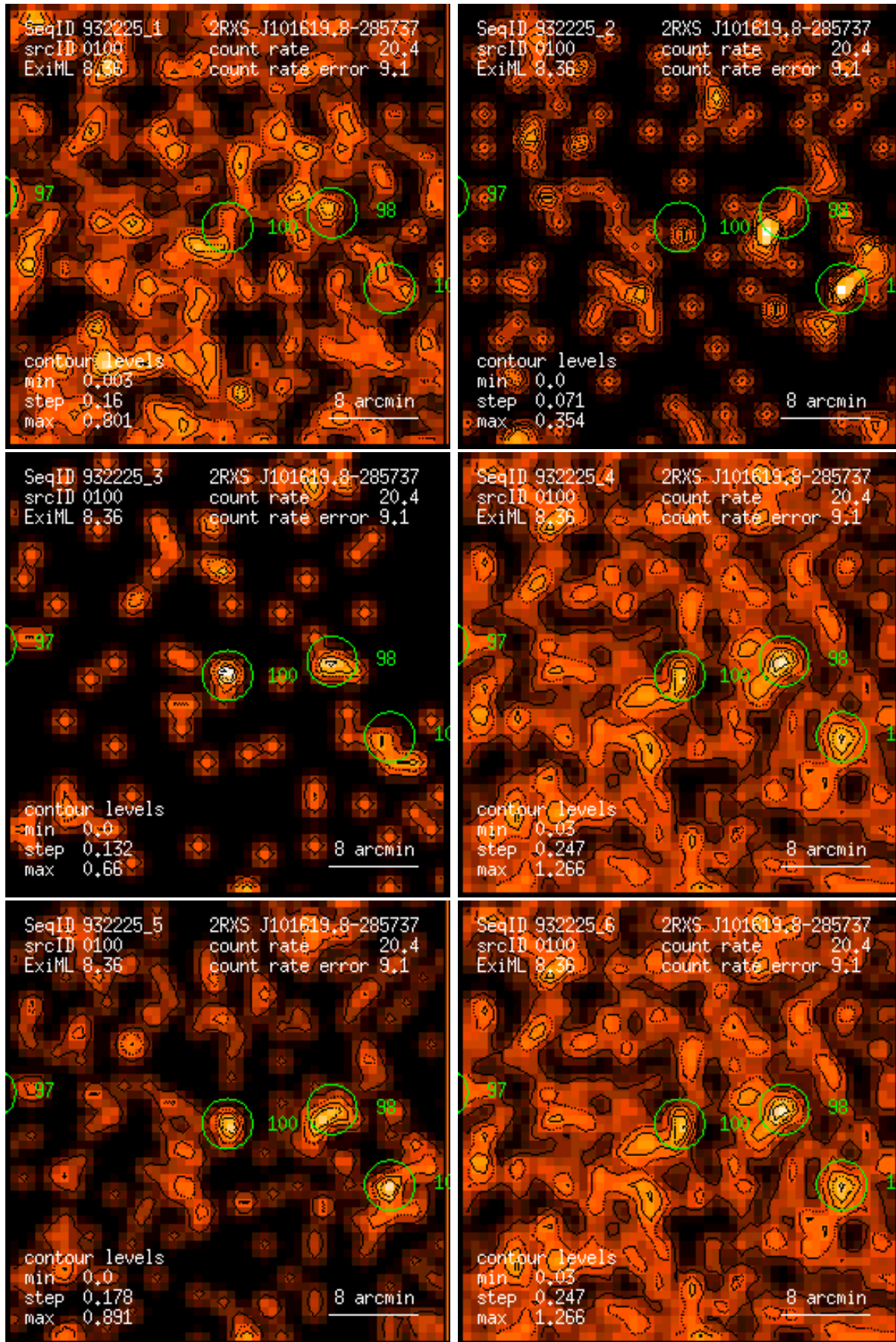
Figure 100: RASS 932225: detection 0100: band rate images, Gaussian filter: (1) PSPC channels 11 – 41, (2) 52 – 90, (3) 91 – 201, (4) 11 – 235, (5) 52 – 201, (6) 11 – 201. Broad band rates in counts/ks. Band rate contour levels in counts/ks/arcmin 2 .
