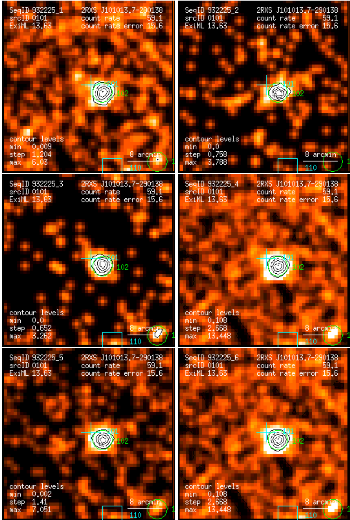
Figure 101: RASS 932225: detection 0101: band rate images, Gaussian filter: (1) PSPC channels 11 – 41, (2) 52 – 90, (3) 91 – 201, (4) 11 – 235, (5) 52 – 201, (6) 11 – 201. Broad band rates in counts/ks. Band rate contour levels in counts/ks/arcmin 2 .
