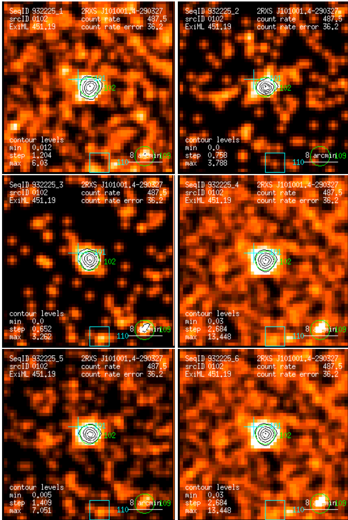
Figure 102: RASS 932225: detection 0102: band rate images, Gaussian filter: (1) PSPC channels 11 – 41, (2) 52 – 90, (3) 91 – 201, (4) 11 – 235, (5) 52 – 201, (6) 11 – 201. Broad band rates in counts/ks. Band rate contour levels in counts/ks/arcmin 2 .
