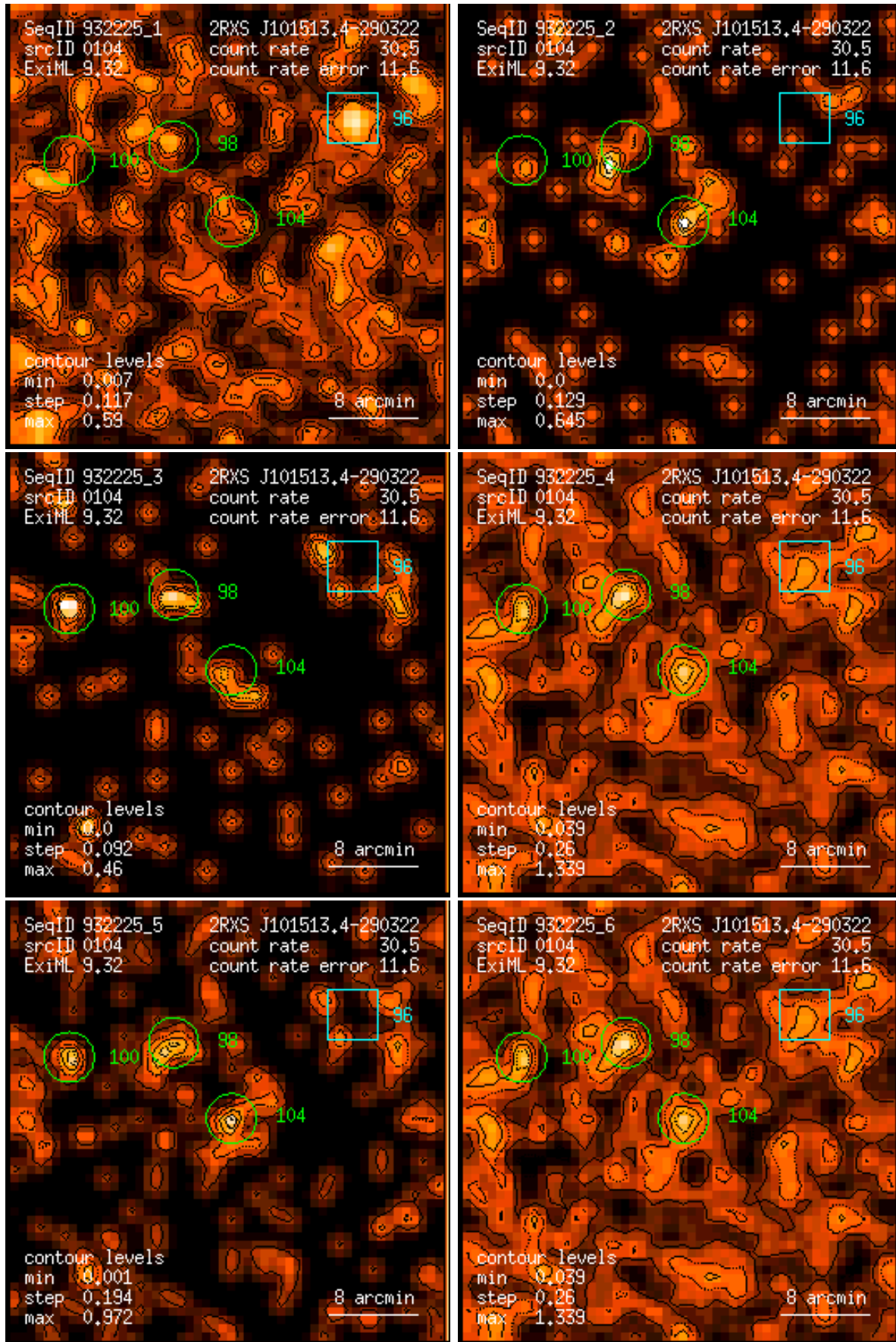
Figure 104: RASS 932225: detection 0104: band rate images, Gaussian filter: (1) PSPC channels 11 – 41, (2) 52 – 90, (3) 91 – 201, (4) 11 – 235, (5) 52 – 201, (6) 11 – 201. Broad band rates in counts/ks. Band rate contour levels in counts/ks/arcmin 2 .
