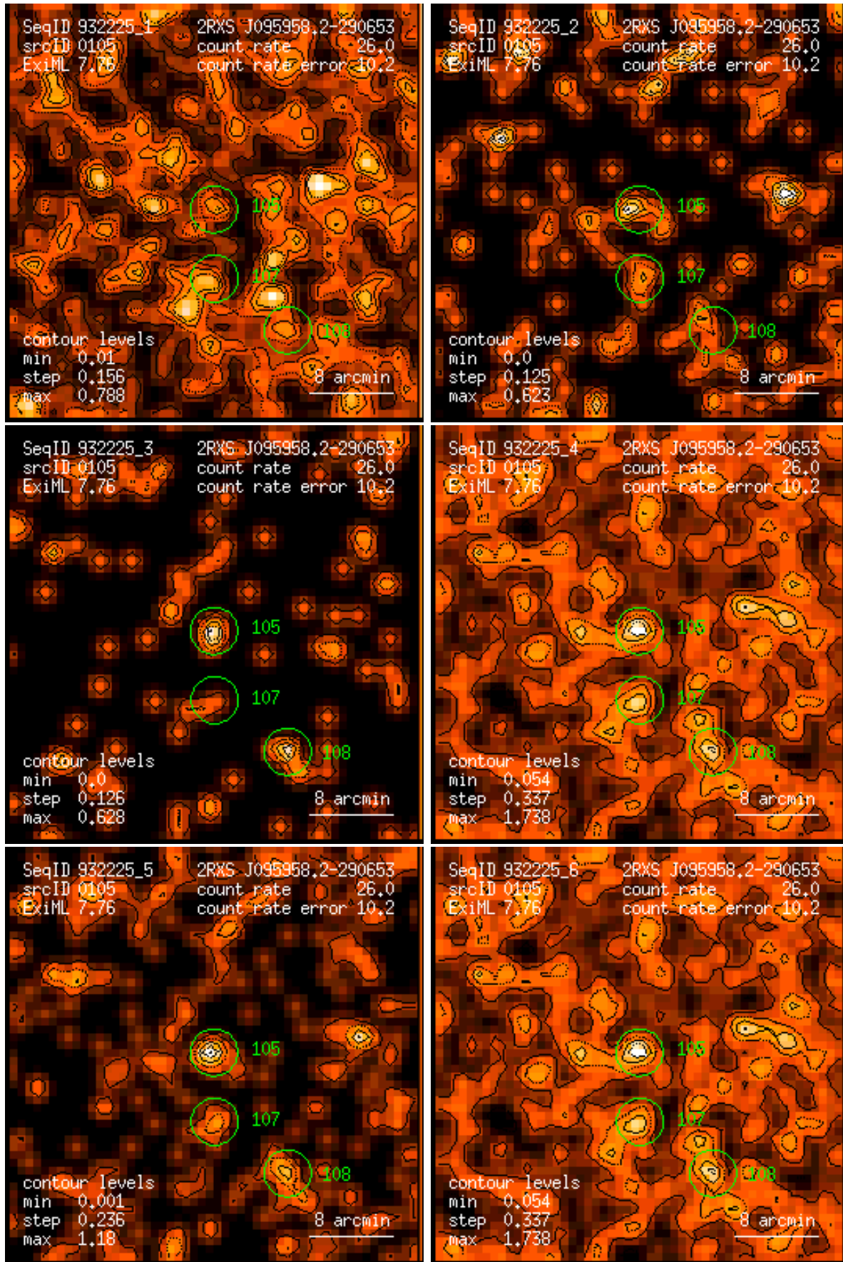
Figure 105: RASS 932225: detection 0105: band rate images, Gaussian filter: (1) PSPC channels 11 – 41, (2) 52 – 90, (3) 91 – 201, (4) 11 – 235, (5) 52 – 201, (6) 11 – 201. Broad band rates in counts/ks. Band rate contour levels in counts/ks/arcmin 2 .
