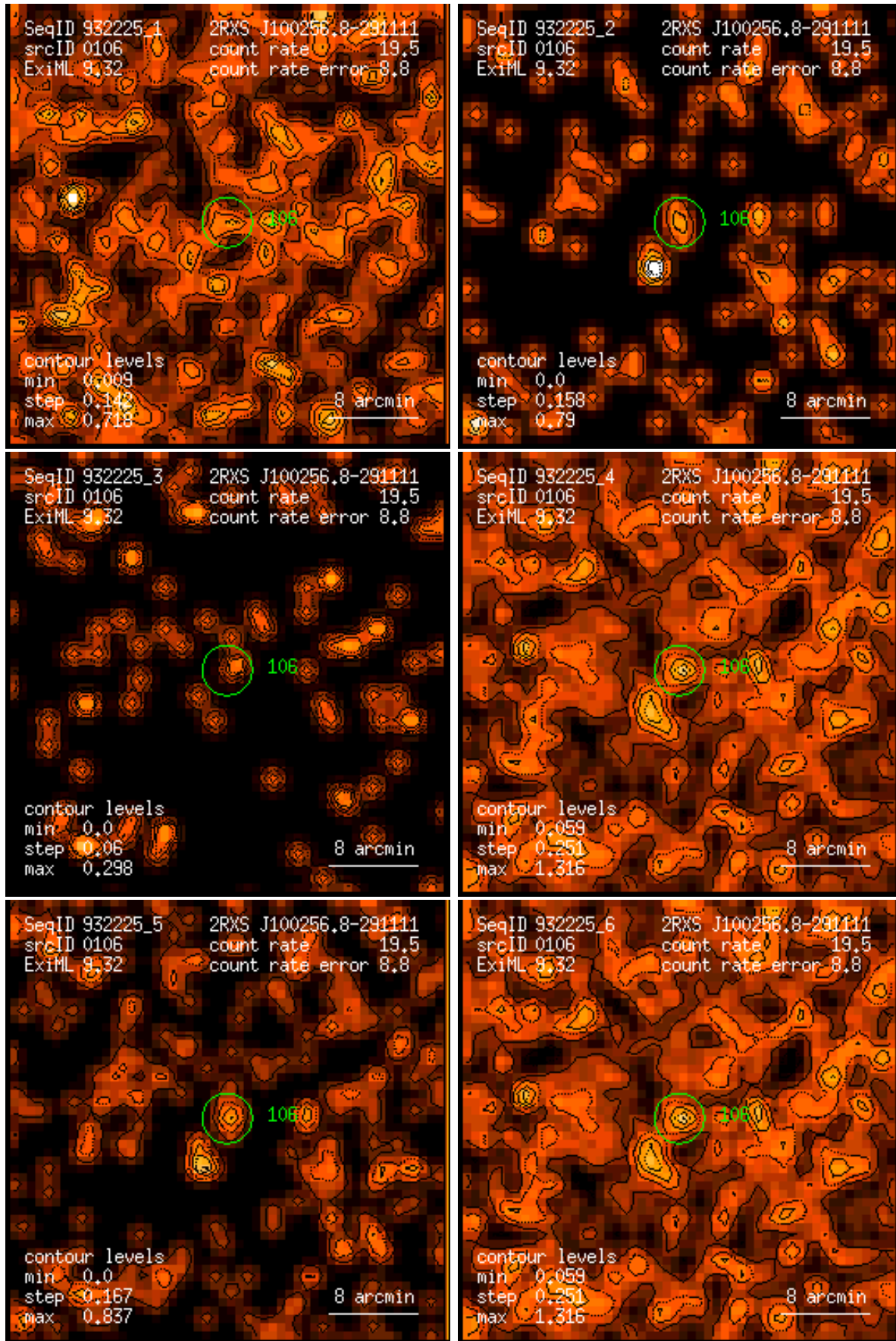
Figure 106: RASS 932225: detection 0106: band rate images, Gaussian filter: (1) PSPC channels 11 – 41, (2) 52 – 90, (3) 91 – 201, (4) 11 – 235, (5) 52 – 201, (6) 11 – 201. Broad band rates in counts/ks. Band rate contour levels in counts/ks/arcmin 2 .
