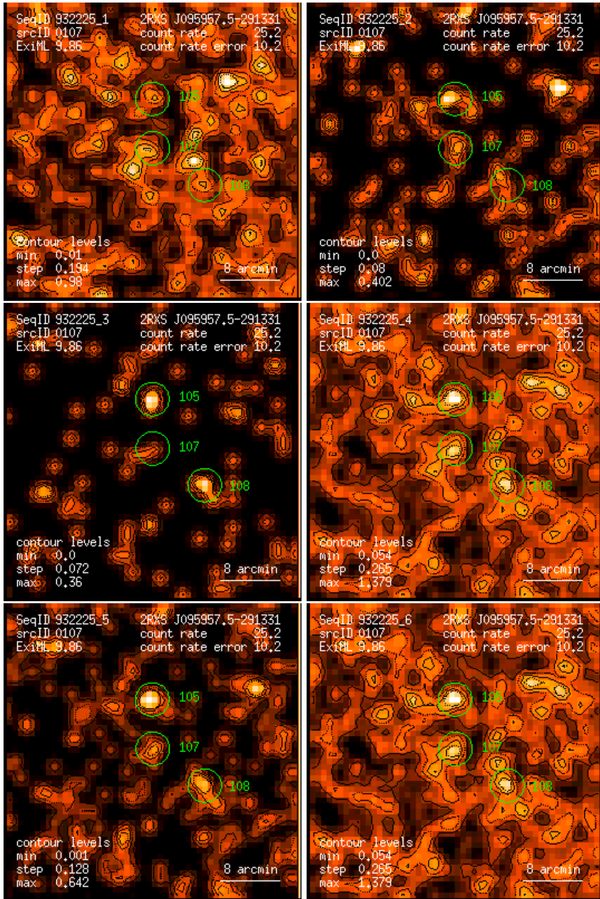
Figure 107: RASS 932225: detection 0107: band rate images, Gaussian filter: (1) PSPC channels 11 – 41, (2) 52 – 90, (3) 91 – 201, (4) 11 – 235, (5) 52 – 201, (6) 11 – 201. Broad band rates in counts/ks. Band rate contour levels in counts/ks/arcmin 2 .
