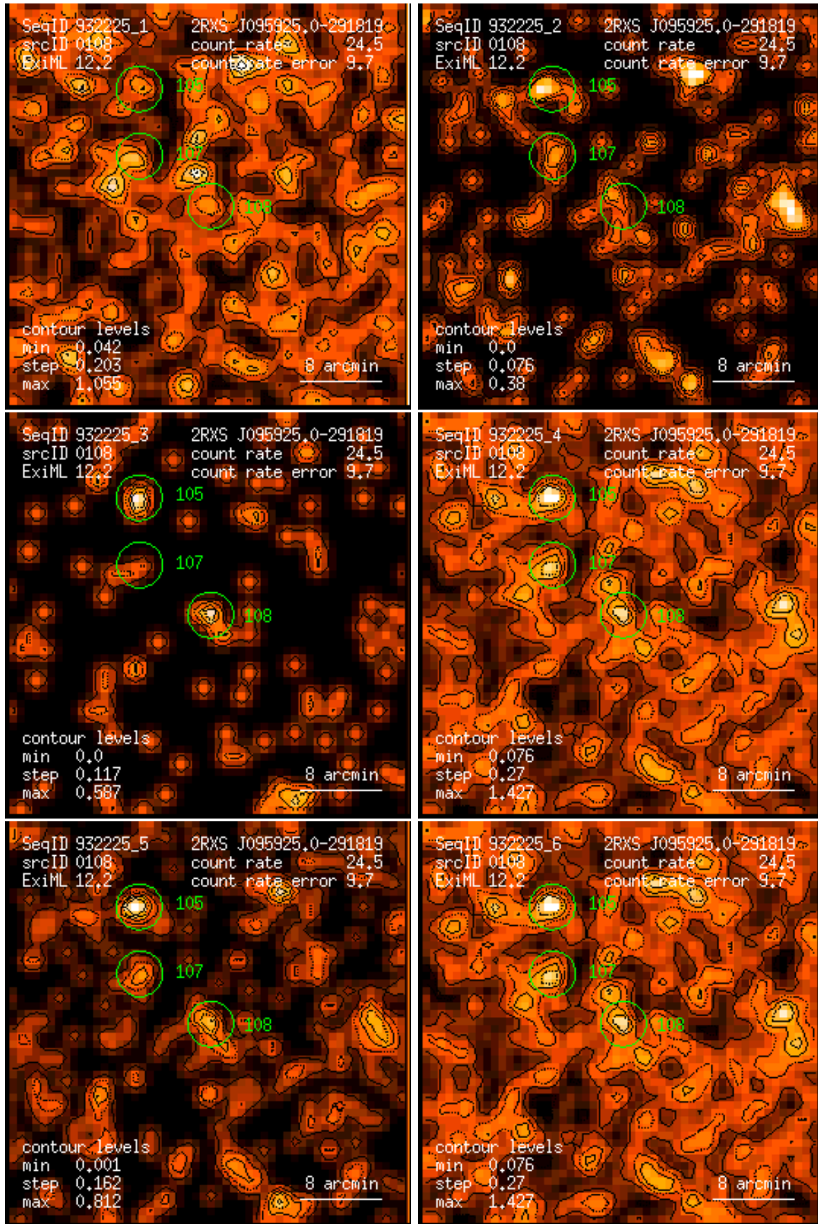
Figure 108: RASS 932225: detection 0108: band rate images, Gaussian filter: (1) PSPC channels 11 – 41, (2) 52 – 90, (3) 91 – 201, (4) 11 – 235, (5) 52 – 201, (6) 11 – 201. Broad band rates in counts/ks. Band rate contour levels in counts/ks/arcmin 2 .
