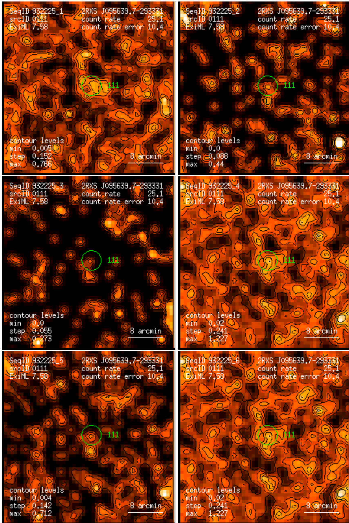
Figure 111: RASS 932225: detection 0111: band rate images, Gaussian filter: (1) PSPC channels 11 – 41, (2) 52 – 90, (3) 91 – 201, (4) 11 – 235, (5) 52 – 201, (6) 11 – 201. Broad band rates in counts/ks. Band rate contour levels in counts/ks/arcmin 2 .
