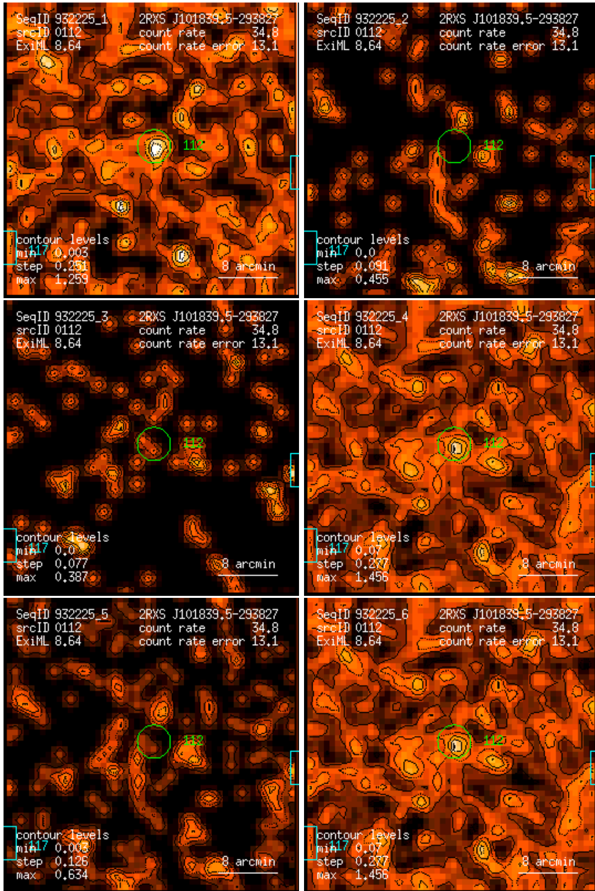
Figure 112: RASS 932225: detection 0112: band rate images, Gaussian filter: (1) PSPC channels 11 – 41, (2) 52 – 90, (3) 91 – 201, (4) 11 – 235, (5) 52 – 201, (6) 11 – 201. Broad band rates in counts/ks. Band rate contour levels in counts/ks/arcmin 2 .
