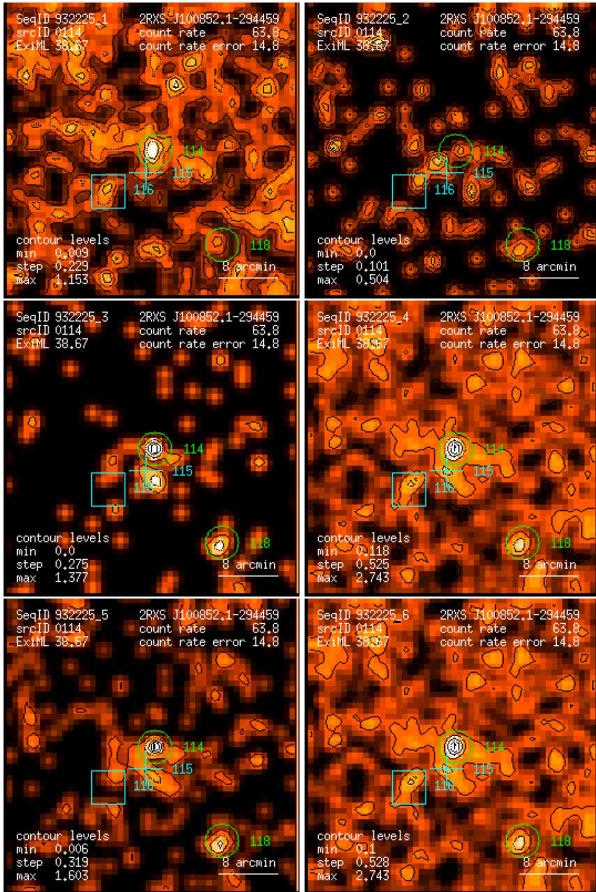
Figure 114: RASS 932225: detection 0114: band rate images, Gaussian filter: (1) PSPC channels 11 – 41, (2) 52 – 90, (3) 91 – 201, (4) 11 – 235, (5) 52 – 201, (6) 11 – 201. Broad band rates in counts/ks. Band rate contour levels in counts/ks/arcmin 2 .
