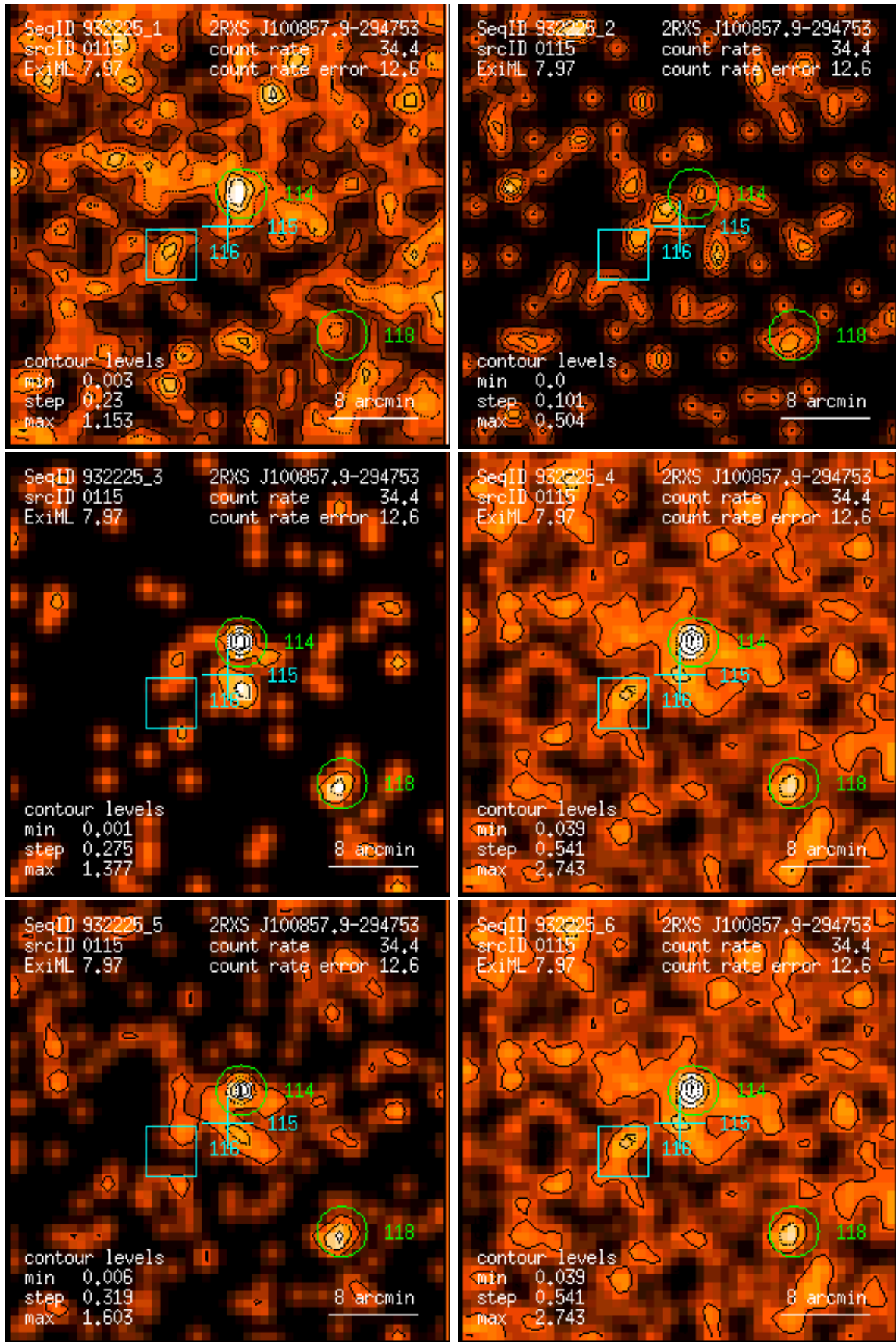
Figure 115: RASS 932225: detection 0115: band rate images, Gaussian filter: (1) PSPC channels 11 – 41, (2) 52 – 90, (3) 91 – 201, (4) 11 – 235, (5) 52 – 201, (6) 11 – 201. Broad band rates in counts/ks. Band rate contour levels in counts/ks/arcmin 2 .
