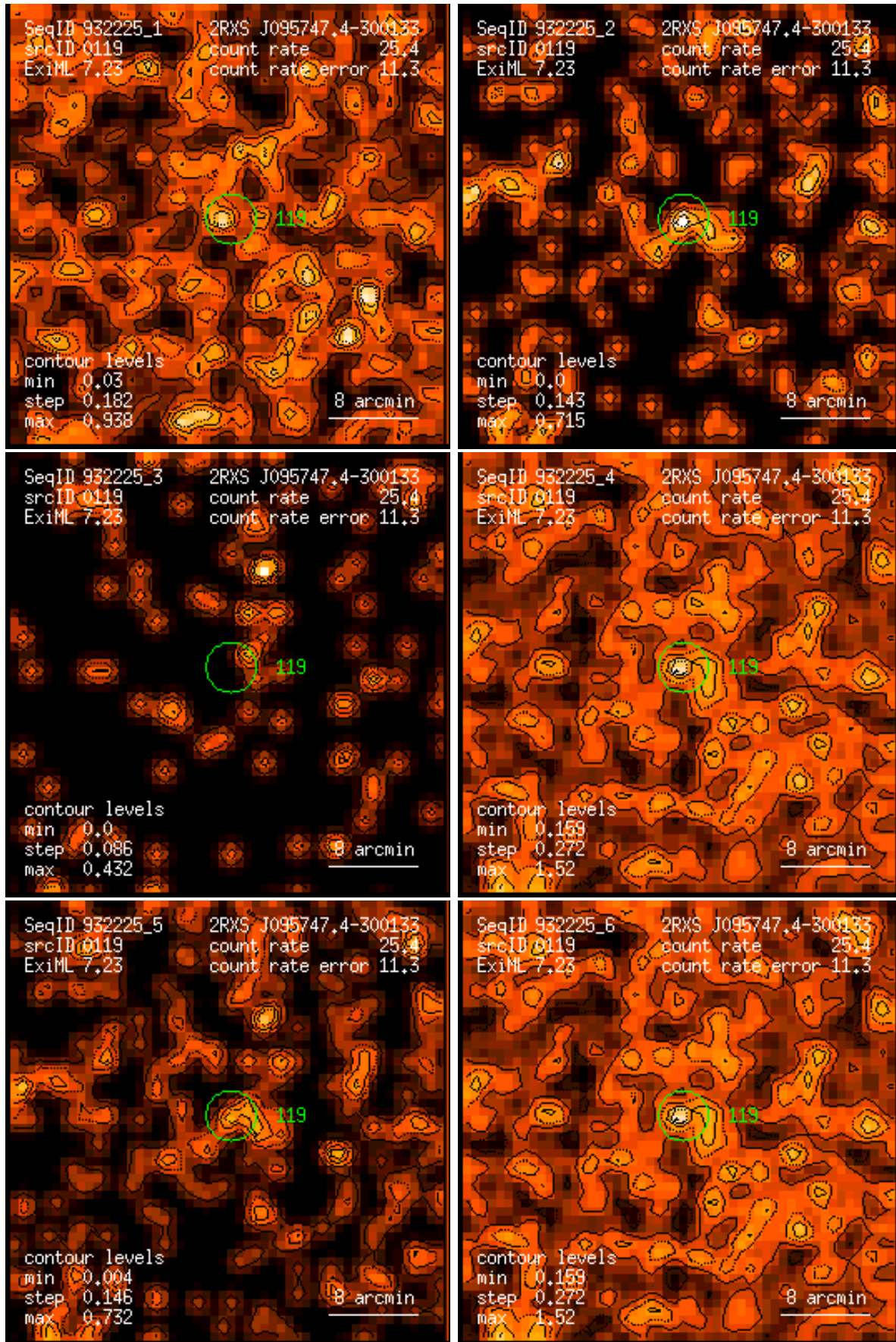
Figure 119: RASS 932225: detection 0119: band rate images, Gaussian filter: (1) PSPC channels 11 – 41, (2) 52 – 90, (3) 91 – 201, (4) 11 – 235, (5) 52 – 201, (6) 11 – 201. Broad band rates in counts/ks. Band rate contour levels in counts/ks/arcmin 2 .
