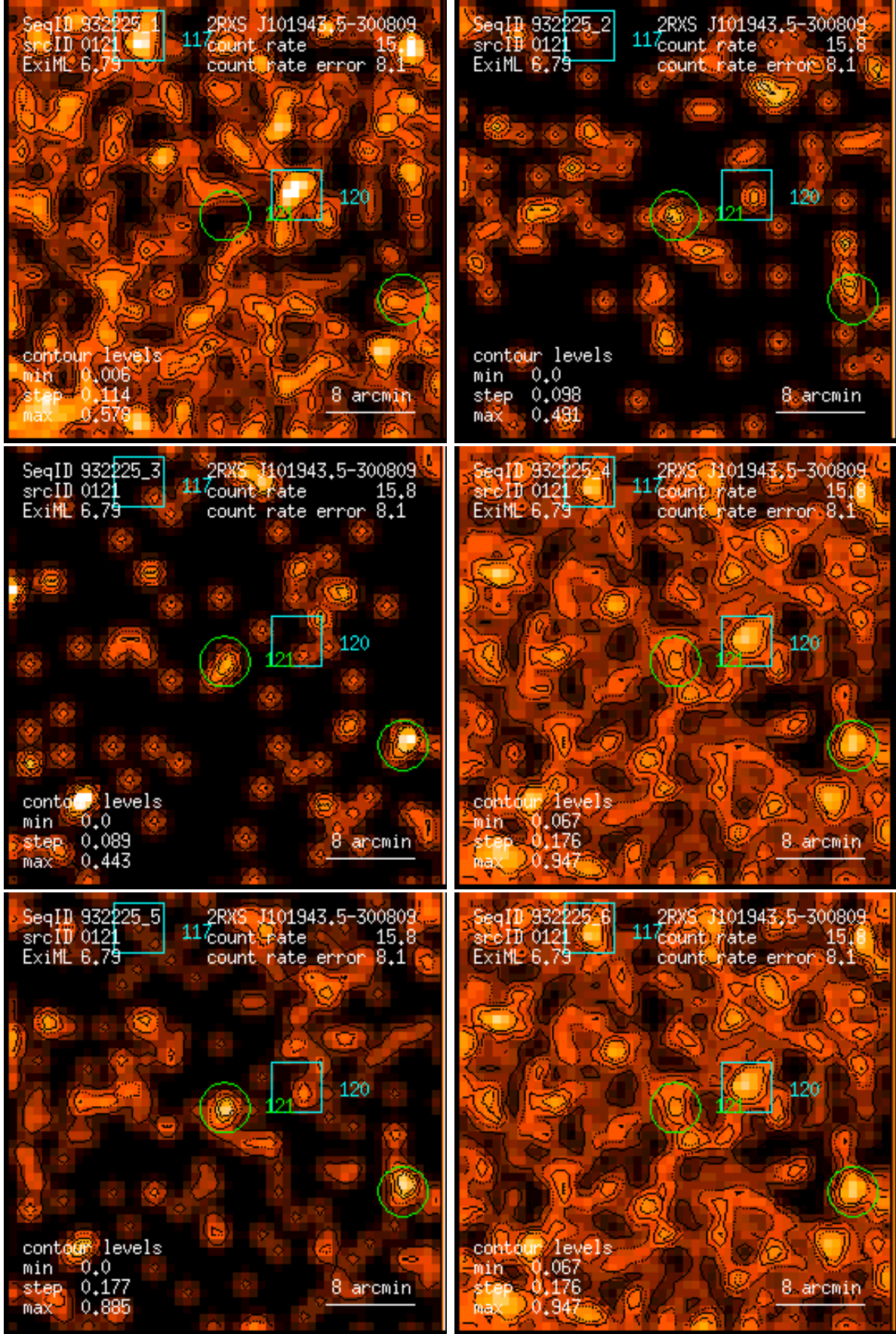
Figure 121: RASS 932225: detection 0121: band rate images, Gaussian filter: (1) PSPC channels 11 – 41, (2) 52 – 90, (3) 91 – 201, (4) 11 – 235, (5) 52 – 201, (6) 11 – 201. Broad band rates in counts/ks. Band rate contour levels in counts/ks/arcmin 2 .
